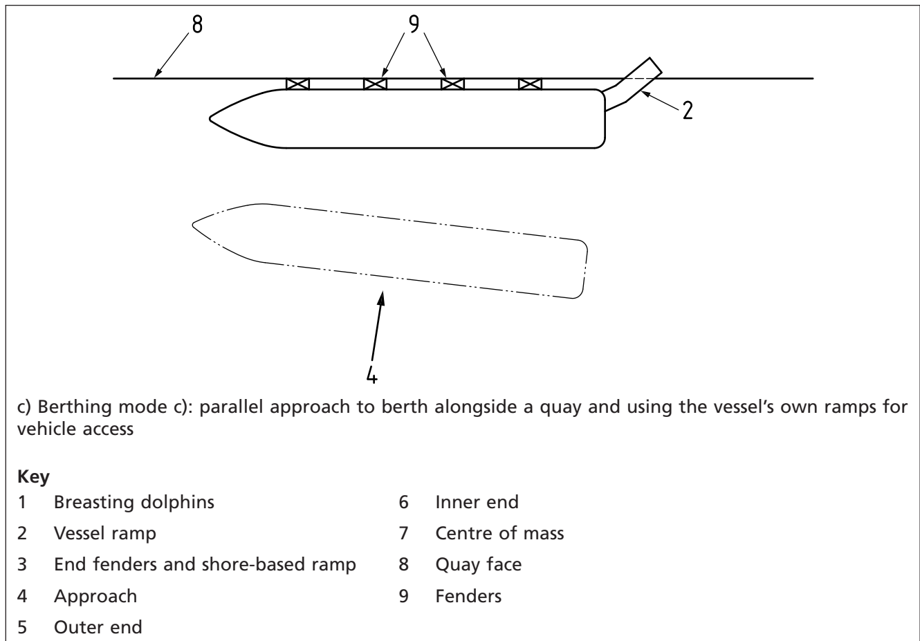
Figure 7 Ferry and Ro-Ro vessel berthing (2 of 2)
