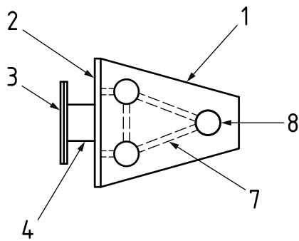
Plan of elastomeric fender a) Flexible dolphin with elastomeric fender
