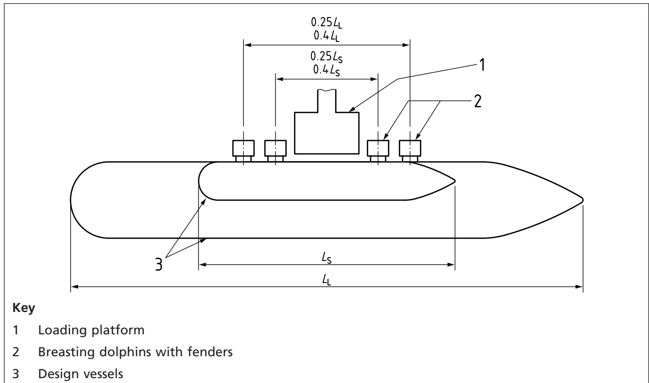
Figure 5 Fender layout for five island berth
