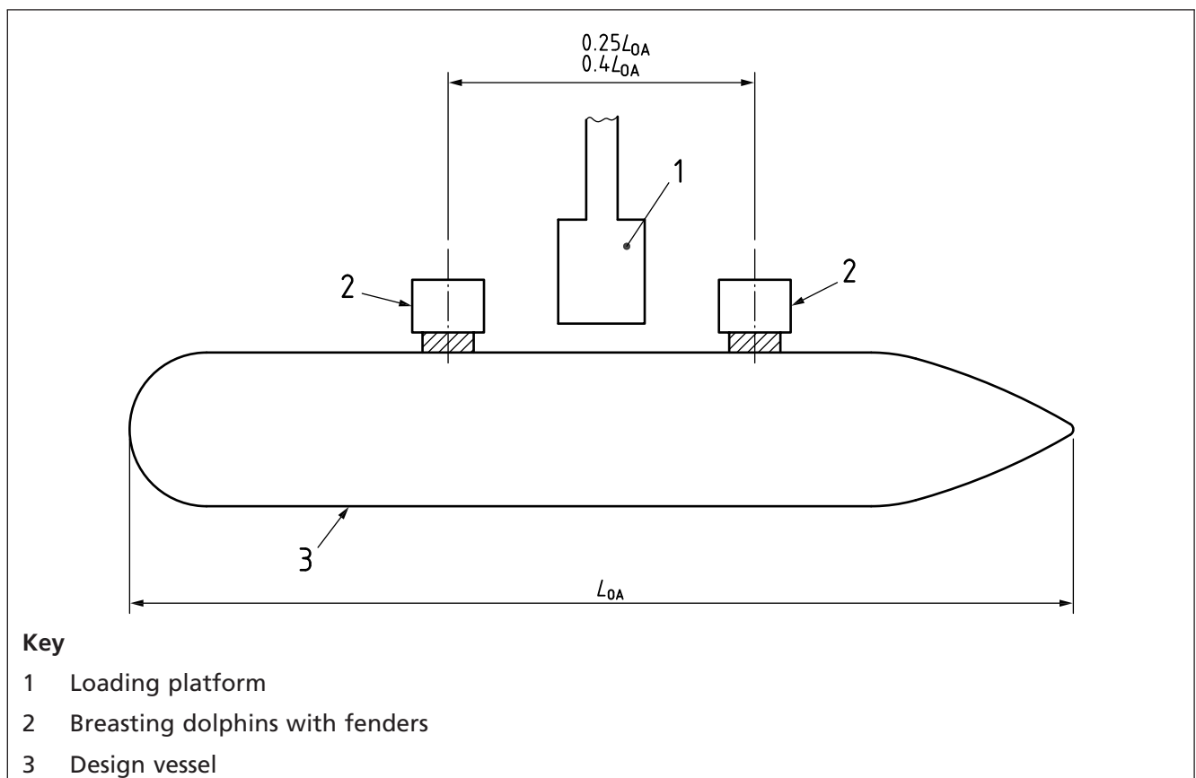
Figure 4 Fender layout for three island berth
