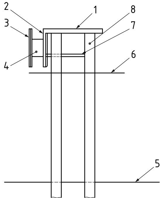
Side elevation of elastomeric fender
