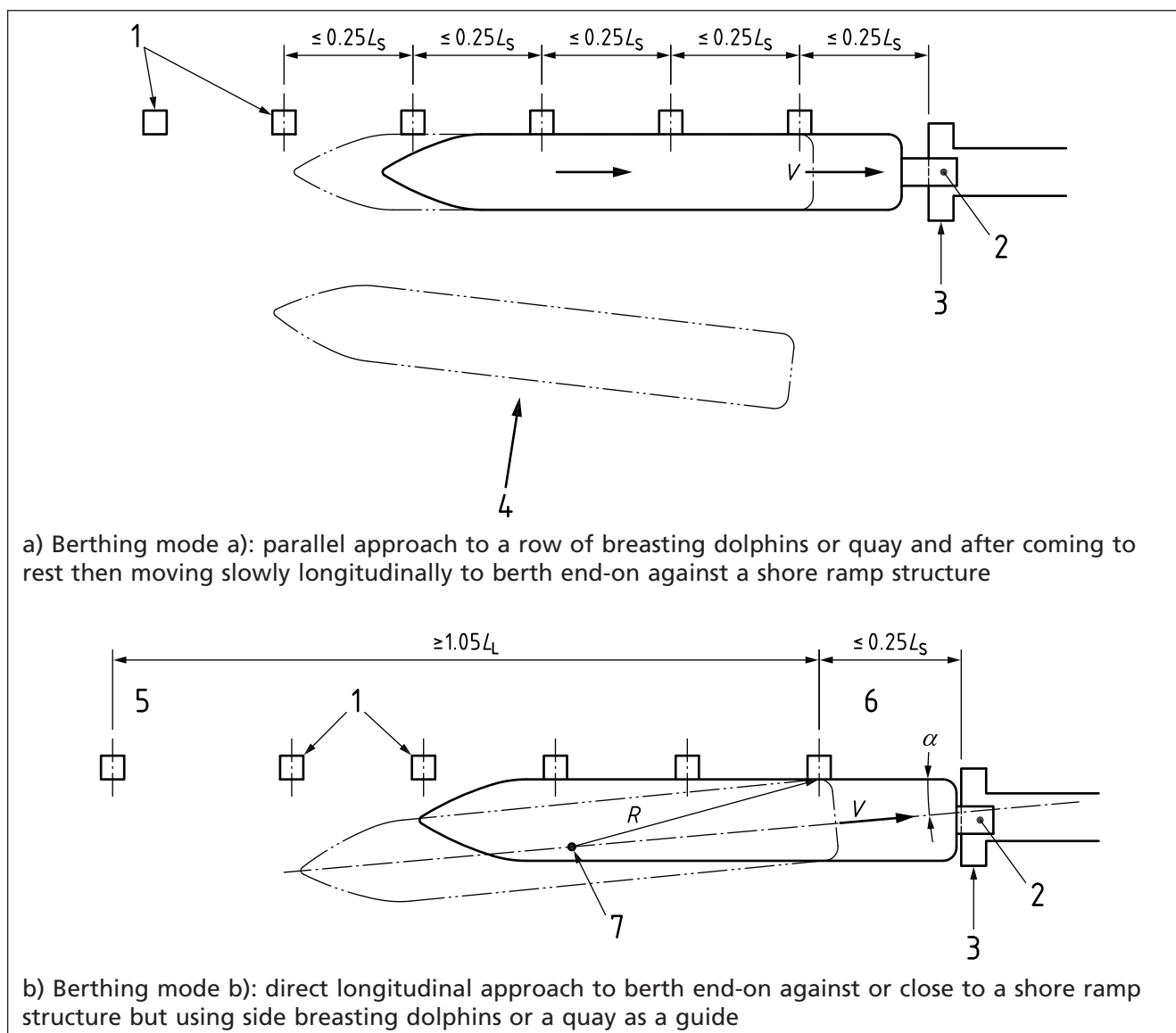
Figure 7 Ferry and Ro-Ro vessel berthing (1 of 2)
