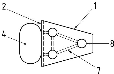
Plan of pneumatic fender b) Flexible dolphin with pneumatic fender
