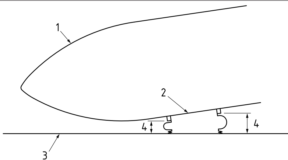
a) Horizontal geometry
