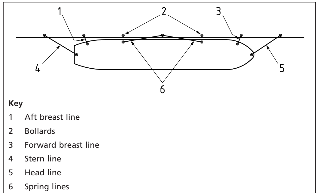
Figure 11 Typical mooring pattern for continuous quay
