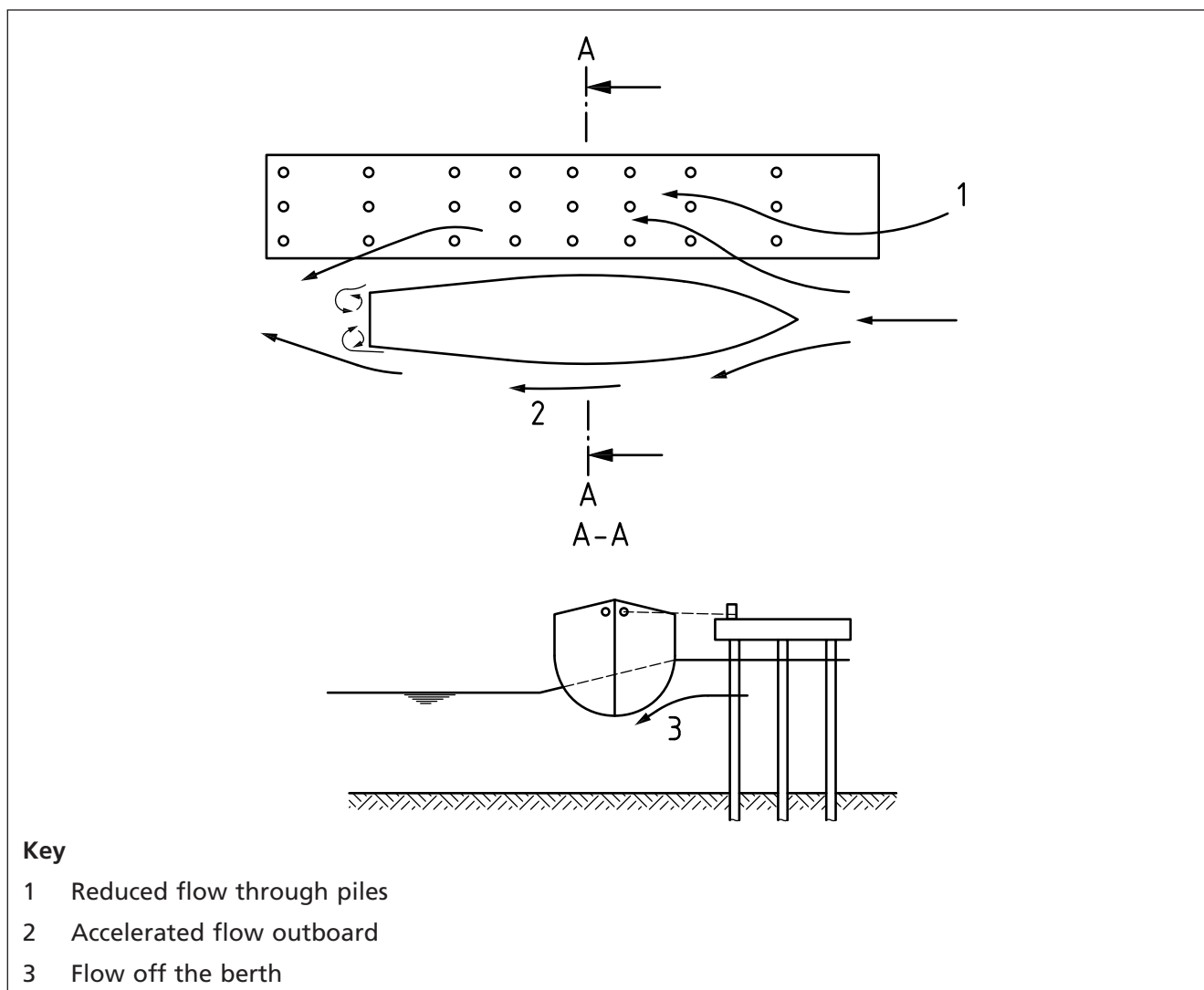
Figure 13 Vessel under influence of stand-off force
