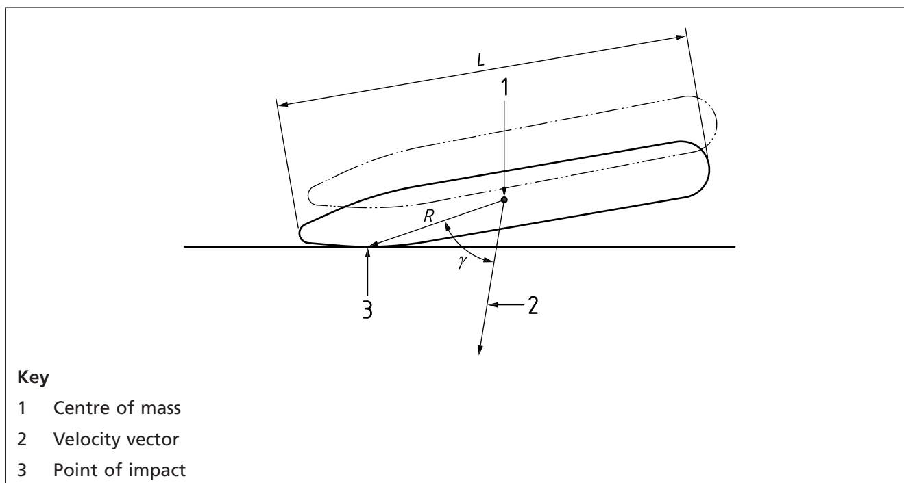
Figure 6 Geometry of vessel approach to berth
