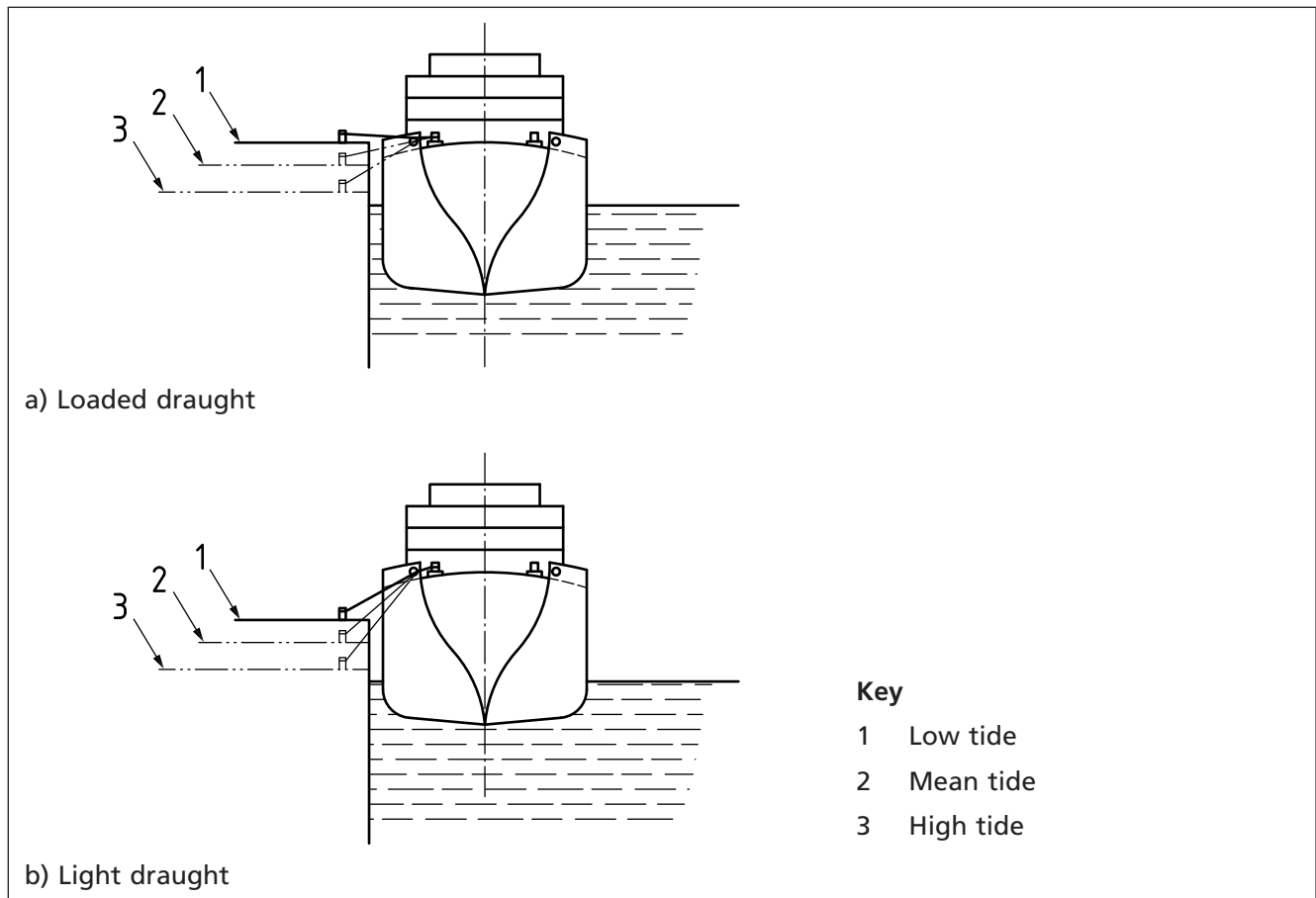
Figure 14 Effect of rise and fall of tide and change in draught or trim
