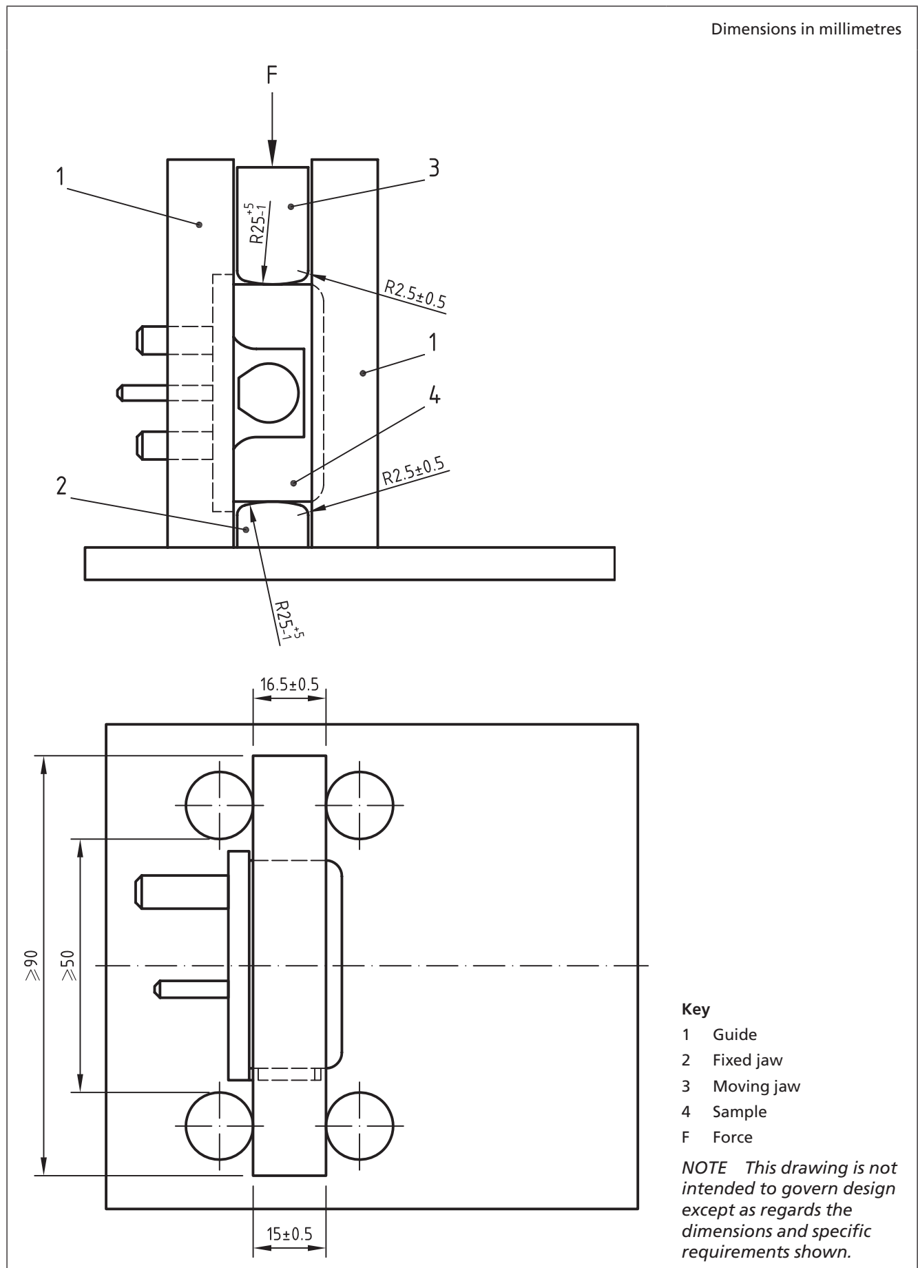
Figure 19 Apparatus for pressure test on portable accessories
