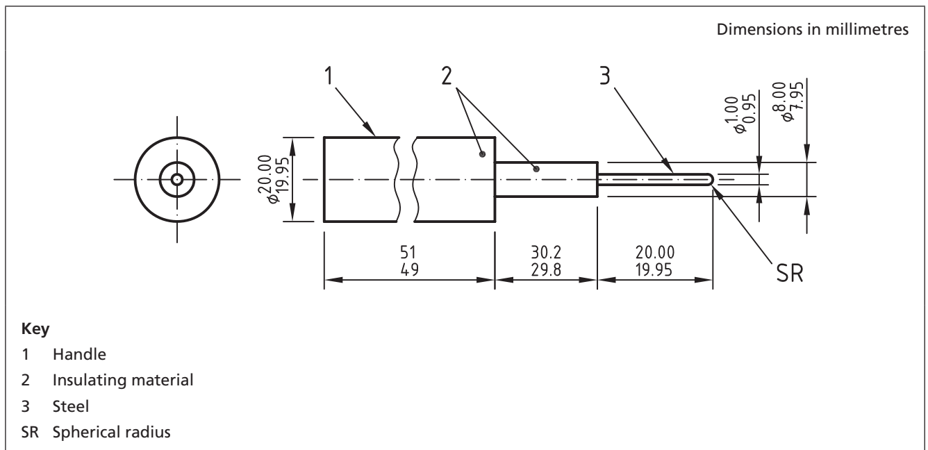
Figure 8 Gauge for checking non-accessibility through shutters
