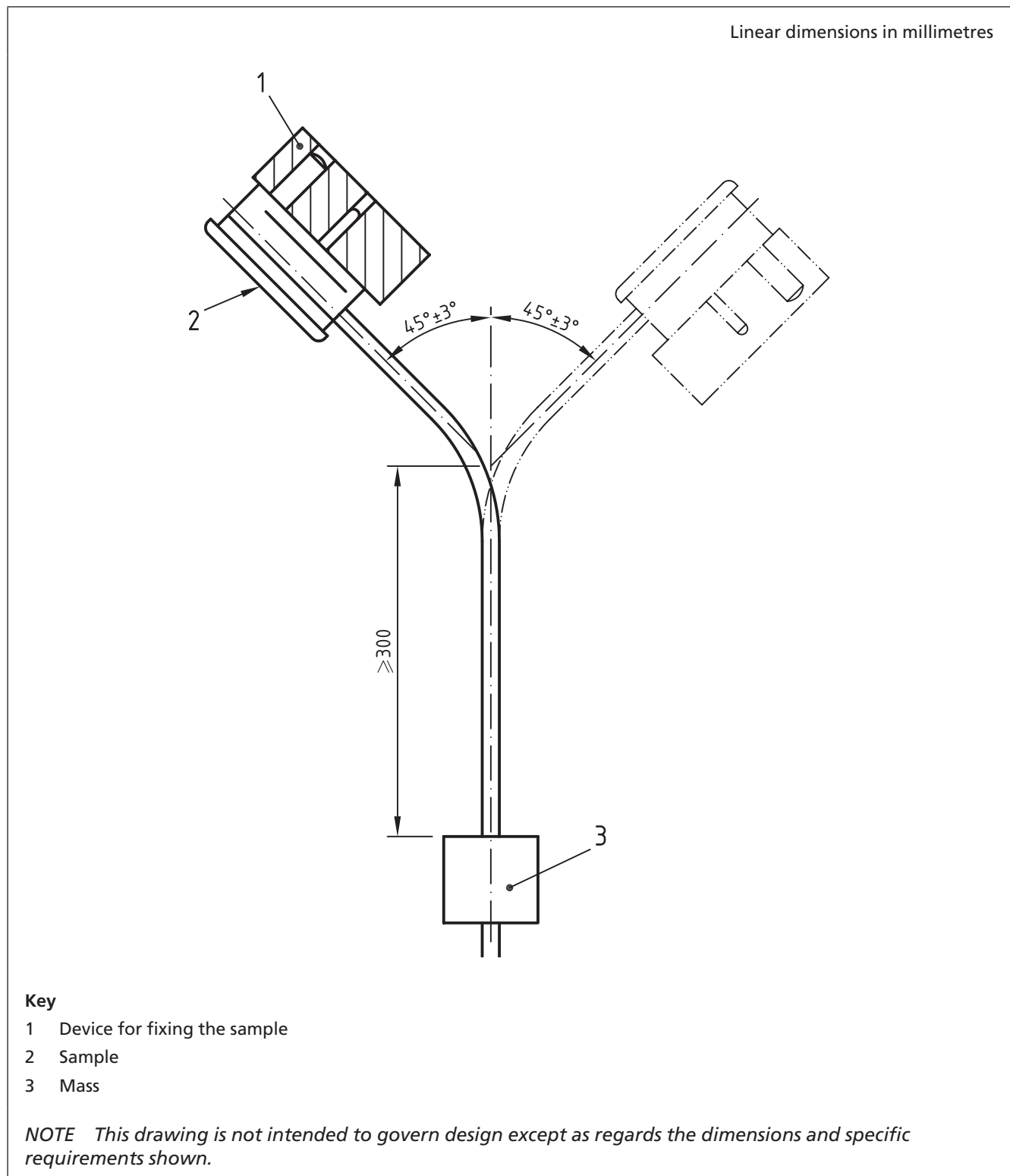
Figure 12 Apparatus for flexing test
