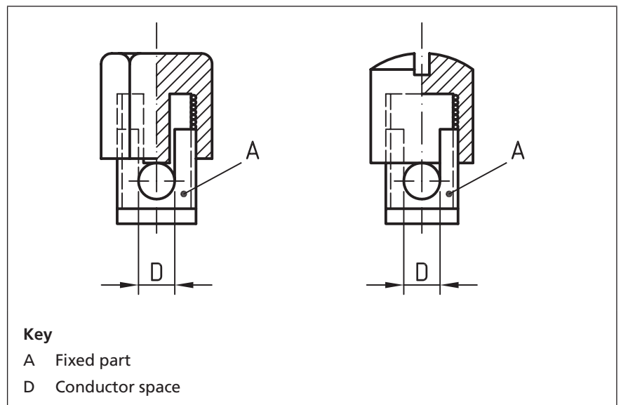
Figure 5 Examples of a mantle terminal
