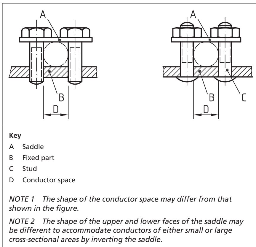
Figure 3 Examples of saddle terminals
