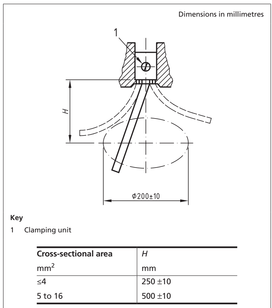
Figure 11 Arrangement for checking damage to conductors
