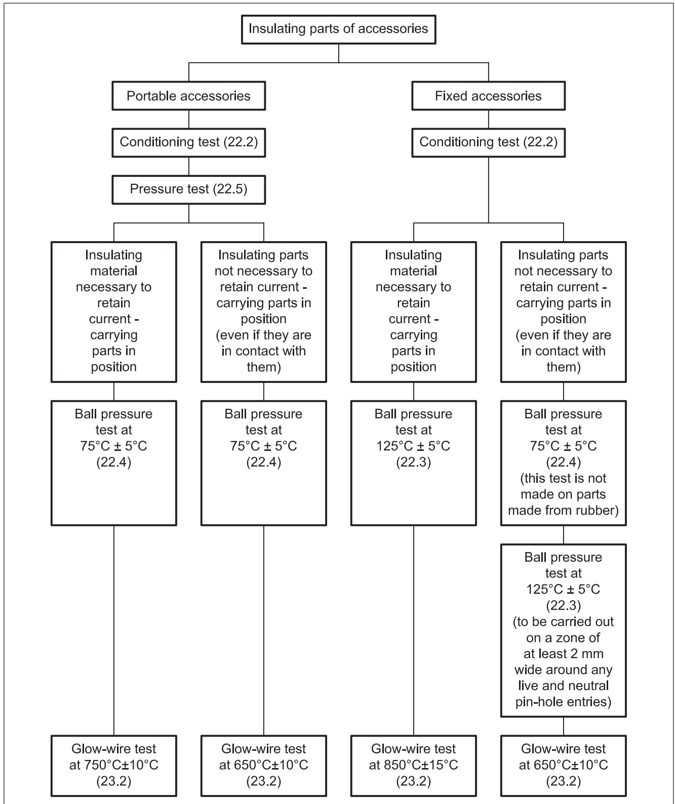
Figure A.1 Diagrammatic representation of the sequence of tests on insulating parts of accessories
