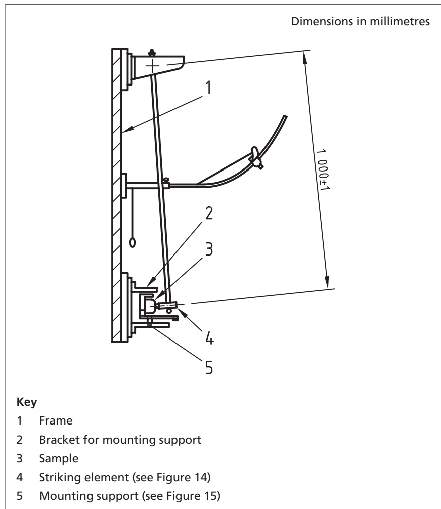
Figure 13 General view of an example of impact test apparatus
