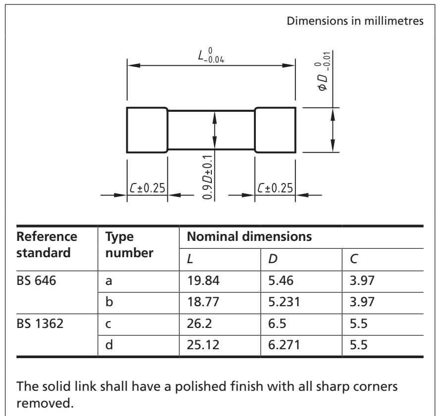
Figure 10 Solid link for test on fuseclips
