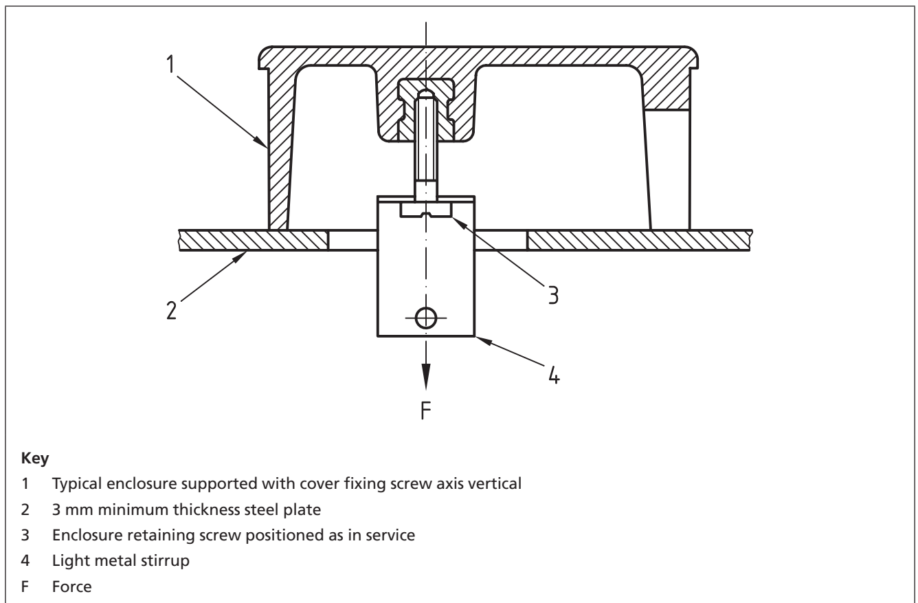
Figure 9 Apparatus for testing accessory enclosure fixing screws
