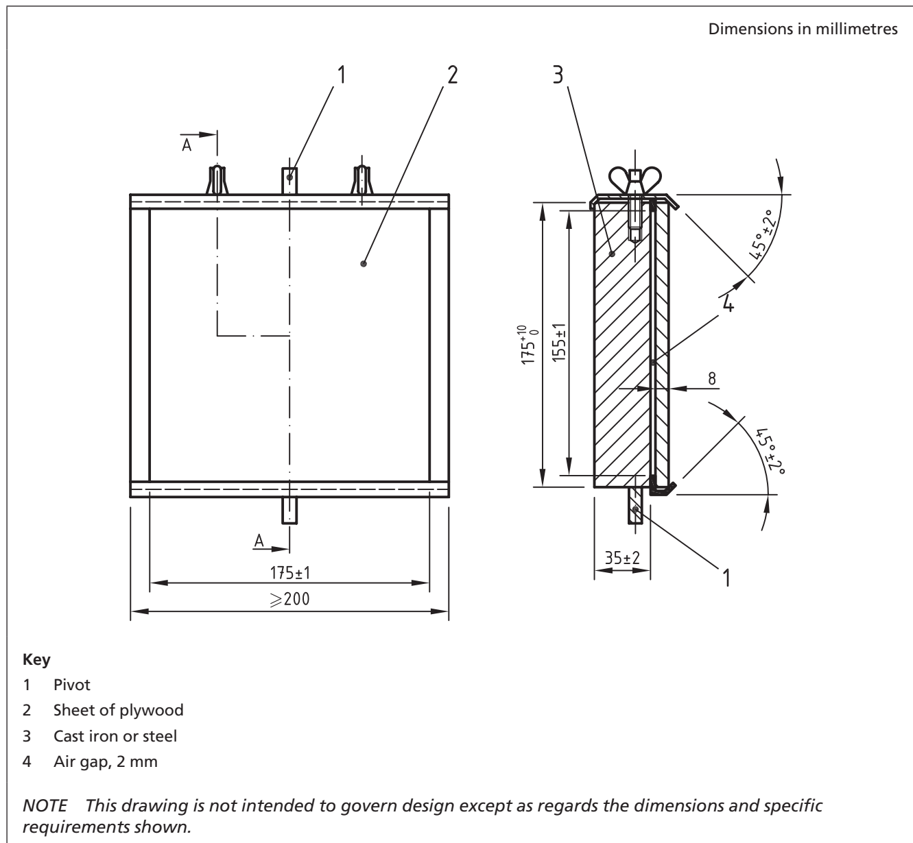
Figure 15 Constructional details of mounting support for test samples
