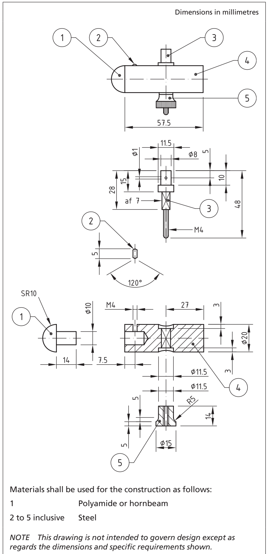
Figure 14 Constructional details of striking element
