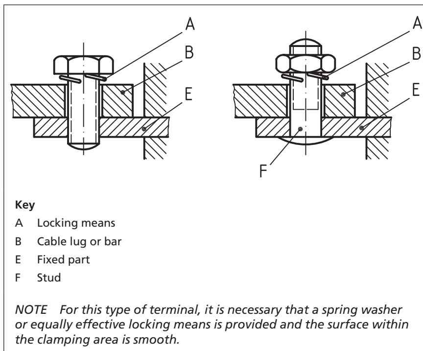
Figure 4 Examples of lug terminals
