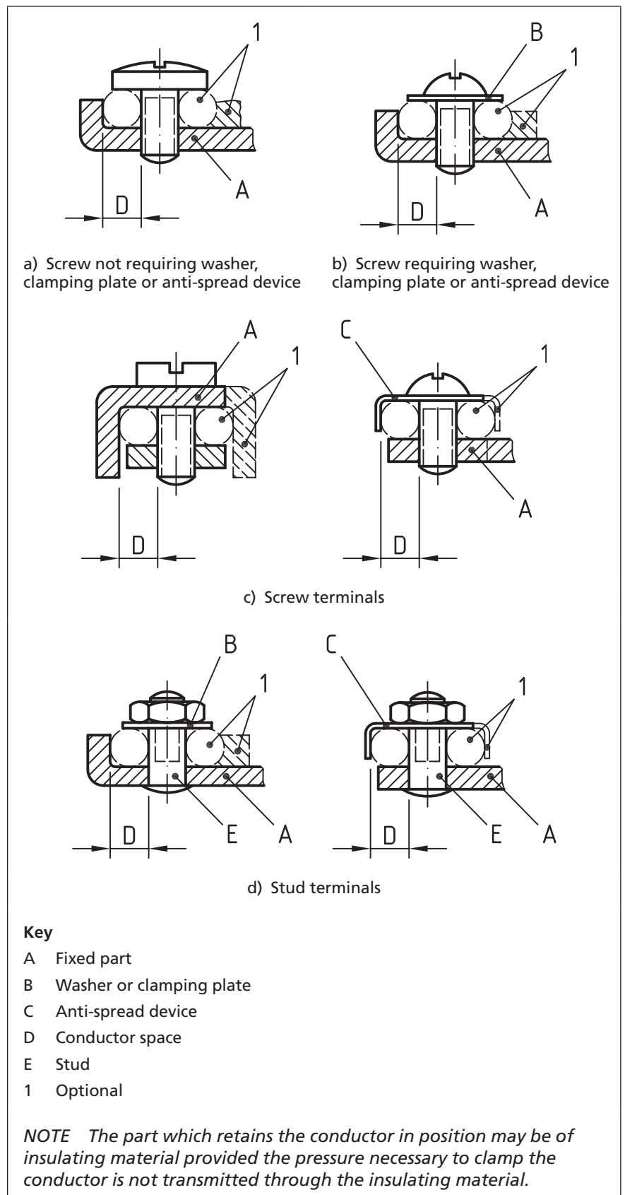
Figure 2 Examples of screw terminals and stud terminals
