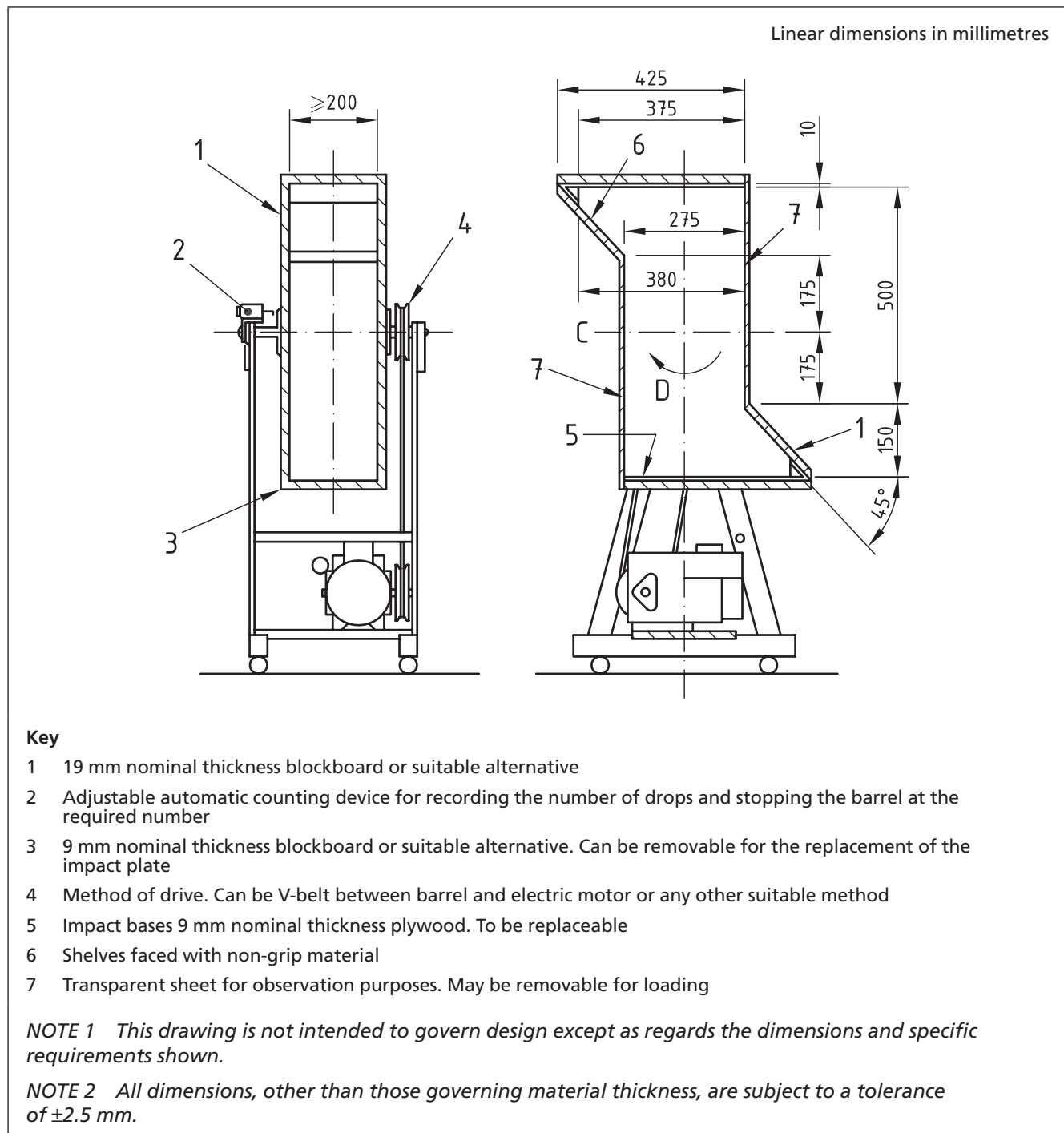
Figure 17 Tumbling barrel
