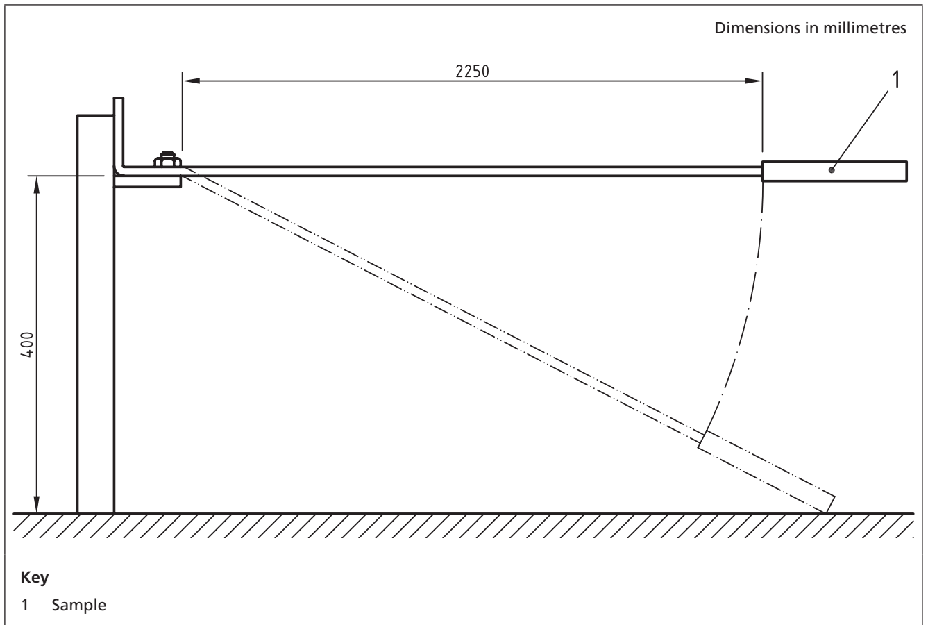
Figure 16 Arrangement for mechanical strength test for portable accessories other than plugs or adaptors
