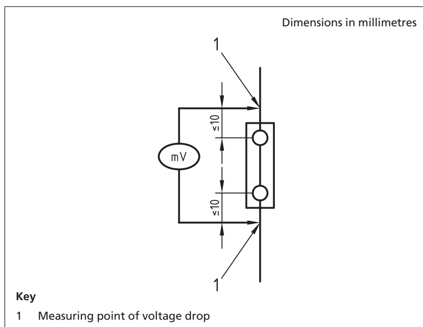
Figure 11A Arrangement for voltage drop test [New Figure]
