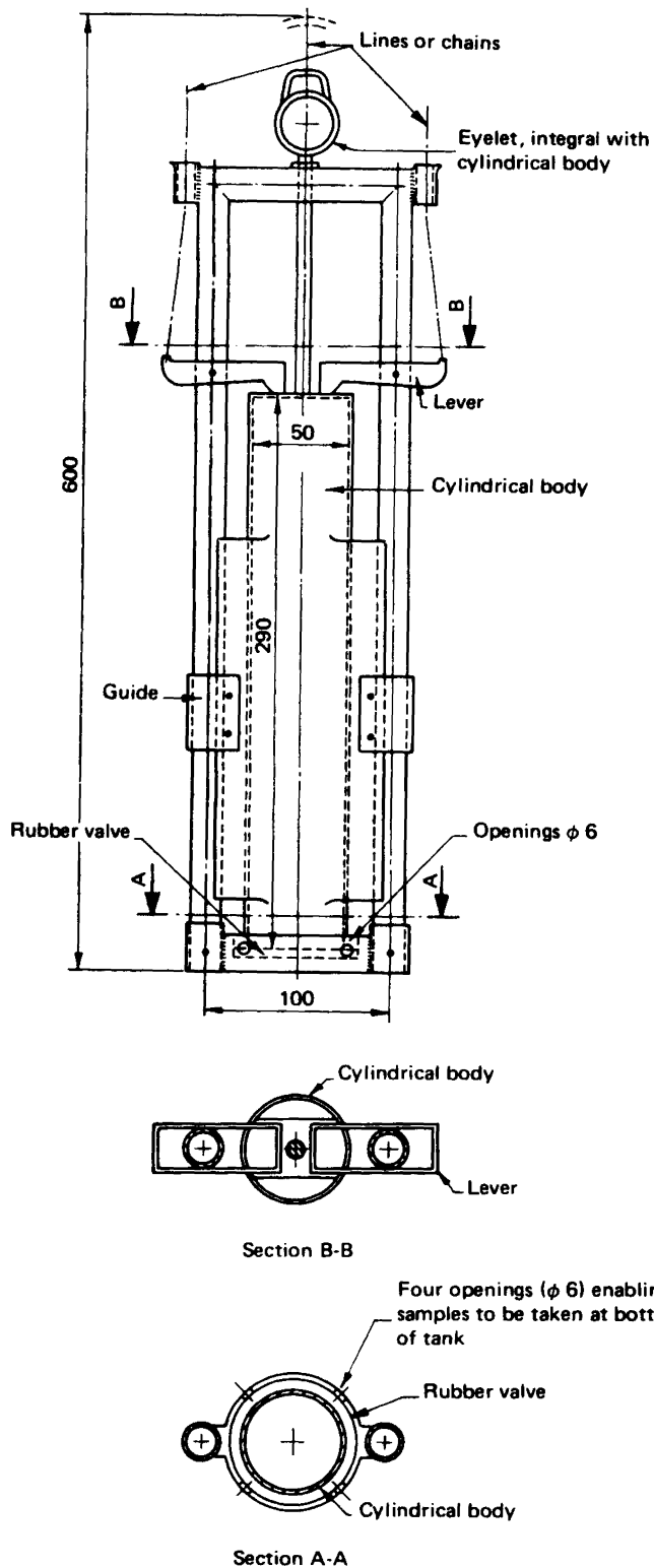
Figure 3 — Example of open-ended cylindrical sampler (6.2.2.1) (Dimensions for guidance only)
