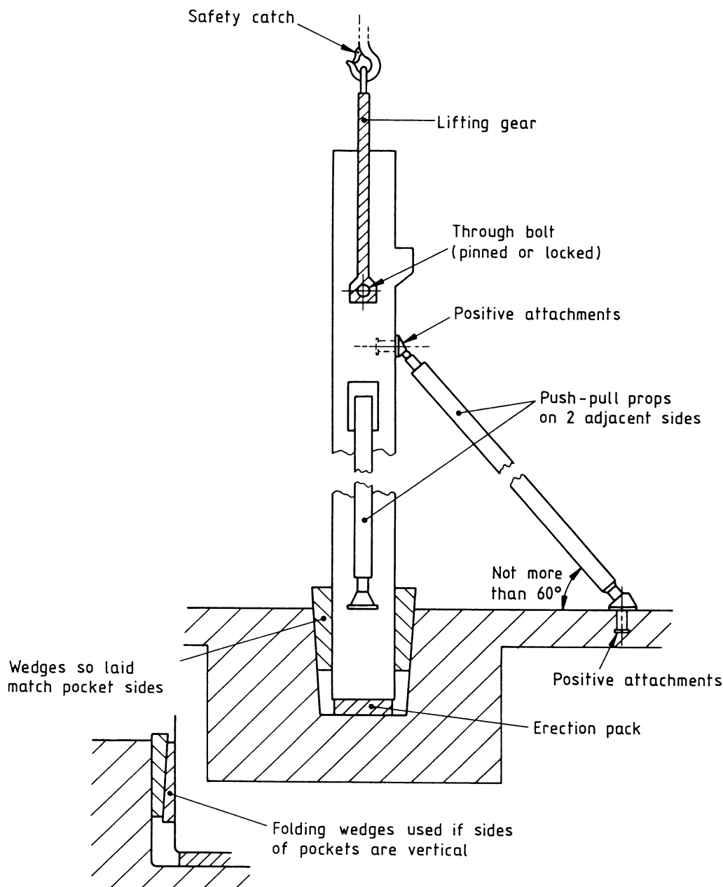
Figure 13 — Precast concrete column: typical bracing arrangement
