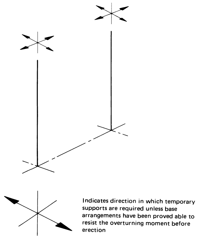
Figure 4 — Stability of single columns (diagrammatic representation)
