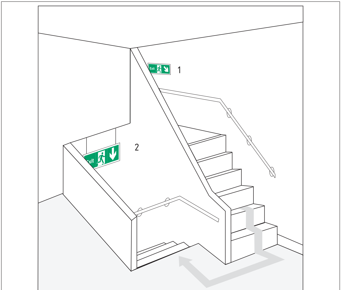
Figure A.3 Typical half landing stairway showing the correct use of escape route sign(s) with supplementary text
