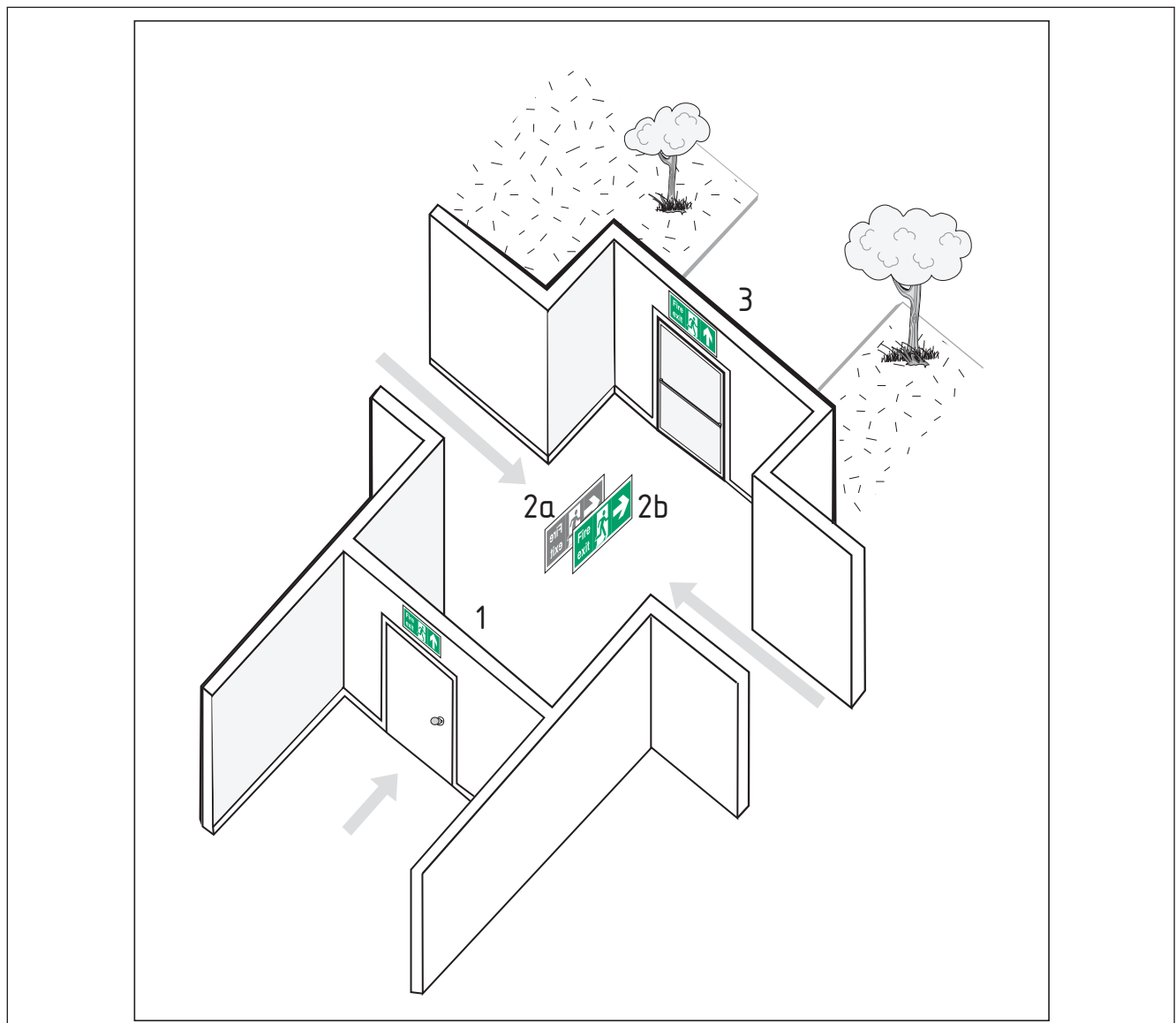
Figure A.5 Typical cross junction/corridor(s) to final fire exit showing the correct use of escape route sign(s) with supplementary text
