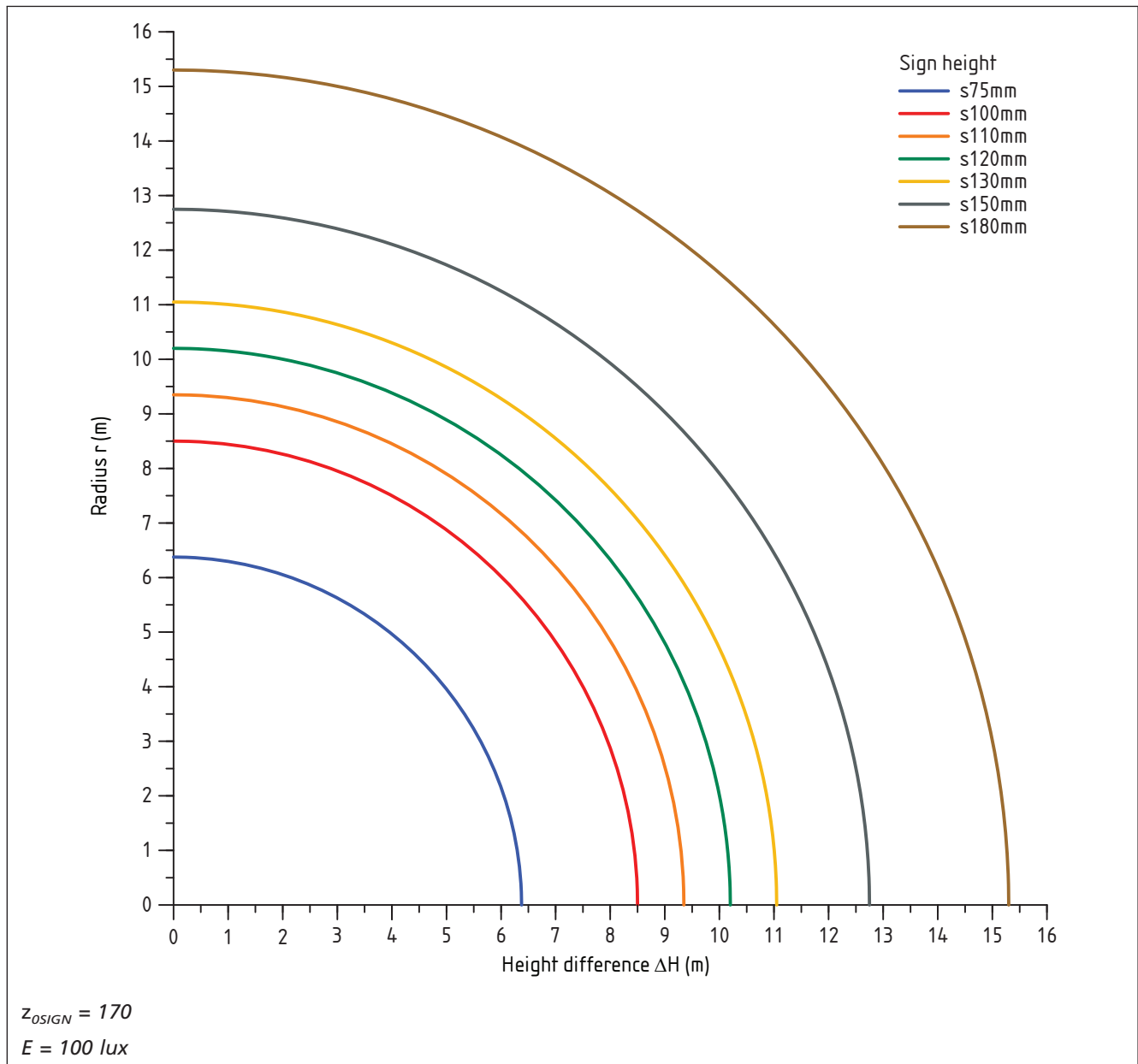
Figure C.2 Variation of radius r against difference in observation height \Delta H for an externally illuminated escape route sign under 100 lux
