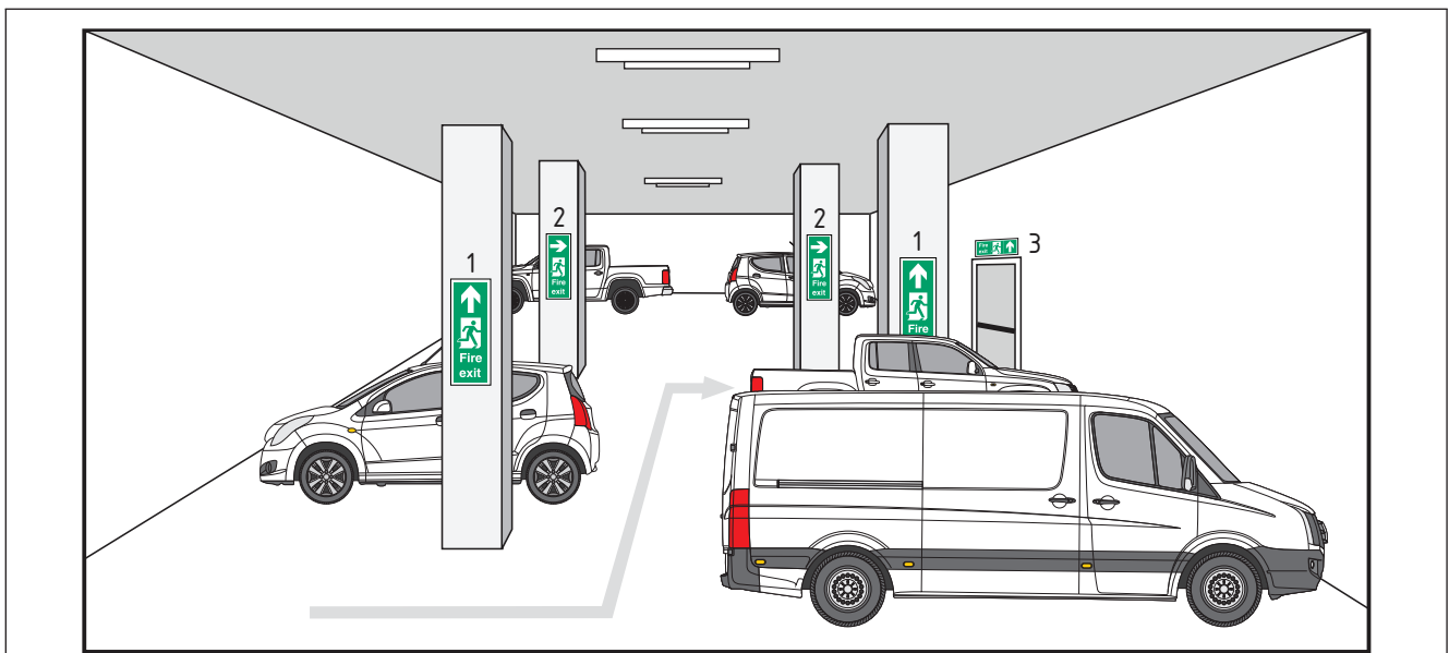
Figure A.15 Typical internal car park progressing forward then right to the final fire exit showing the correct use of escape route sign(s) with supplementary text
