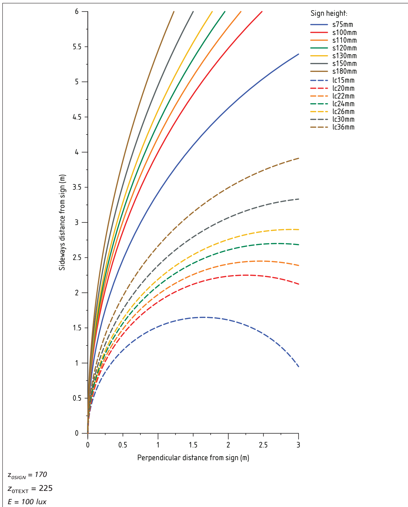
Figure C.5 Circular boundaries of observation distances for escape route sign and lower case supplementary text in horizontal plane: vertical illuminance 100 lux
