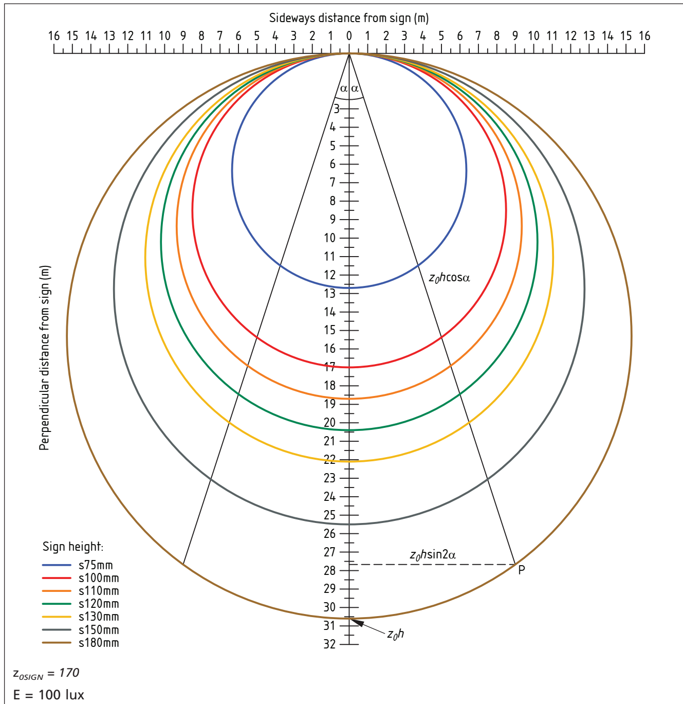
Figure C.1 Circular boundaries of observation distances in horizontal plane
