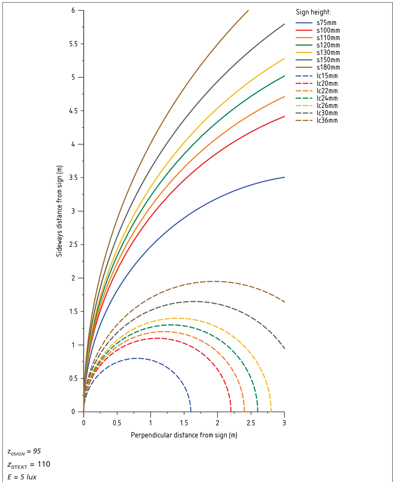
Figure C.7 Circular boundaries of observation distances for escape route sign and lower case supplementary text in horizontal plane: vertical illuminance 5 lux
