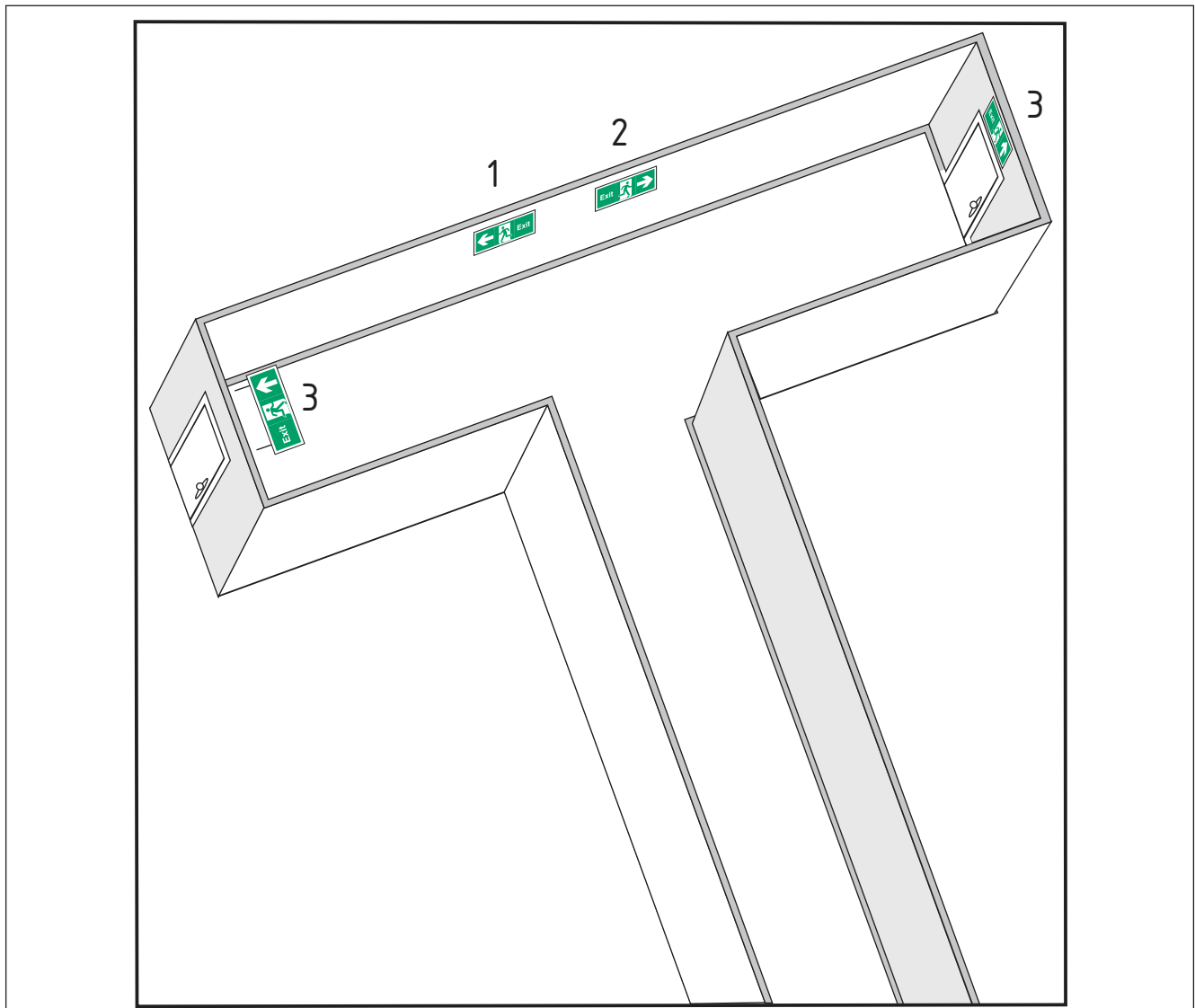
Figure A.19 Typical T-junction corridor offering alternate equidistant routes showing the correct use of escape route sign(s) and supplementary text
