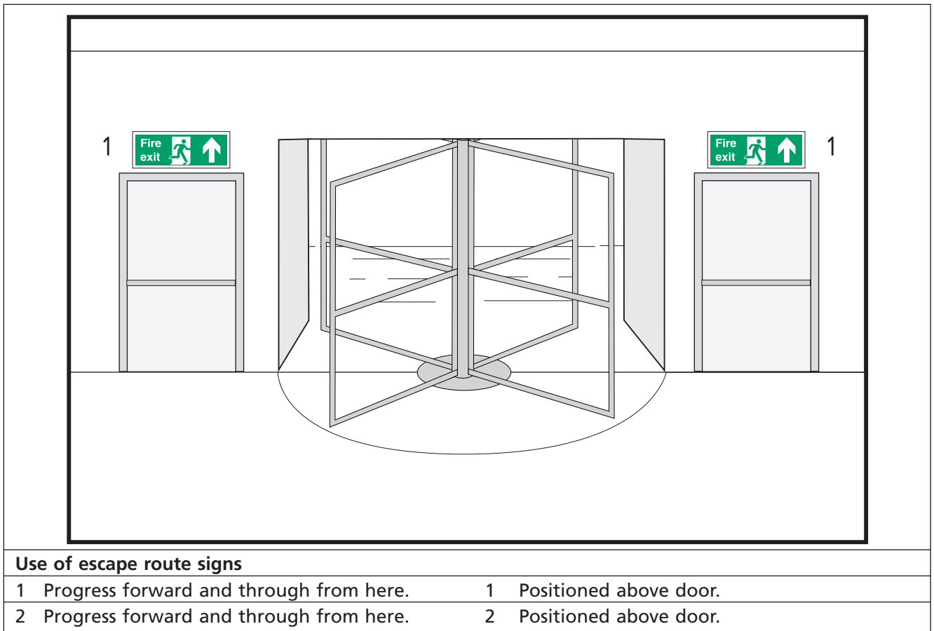
Figure A.22 Typical revolving door arrangement showing the identification of fire exit(s) with the use of escape route sign(s) and supplementary text
