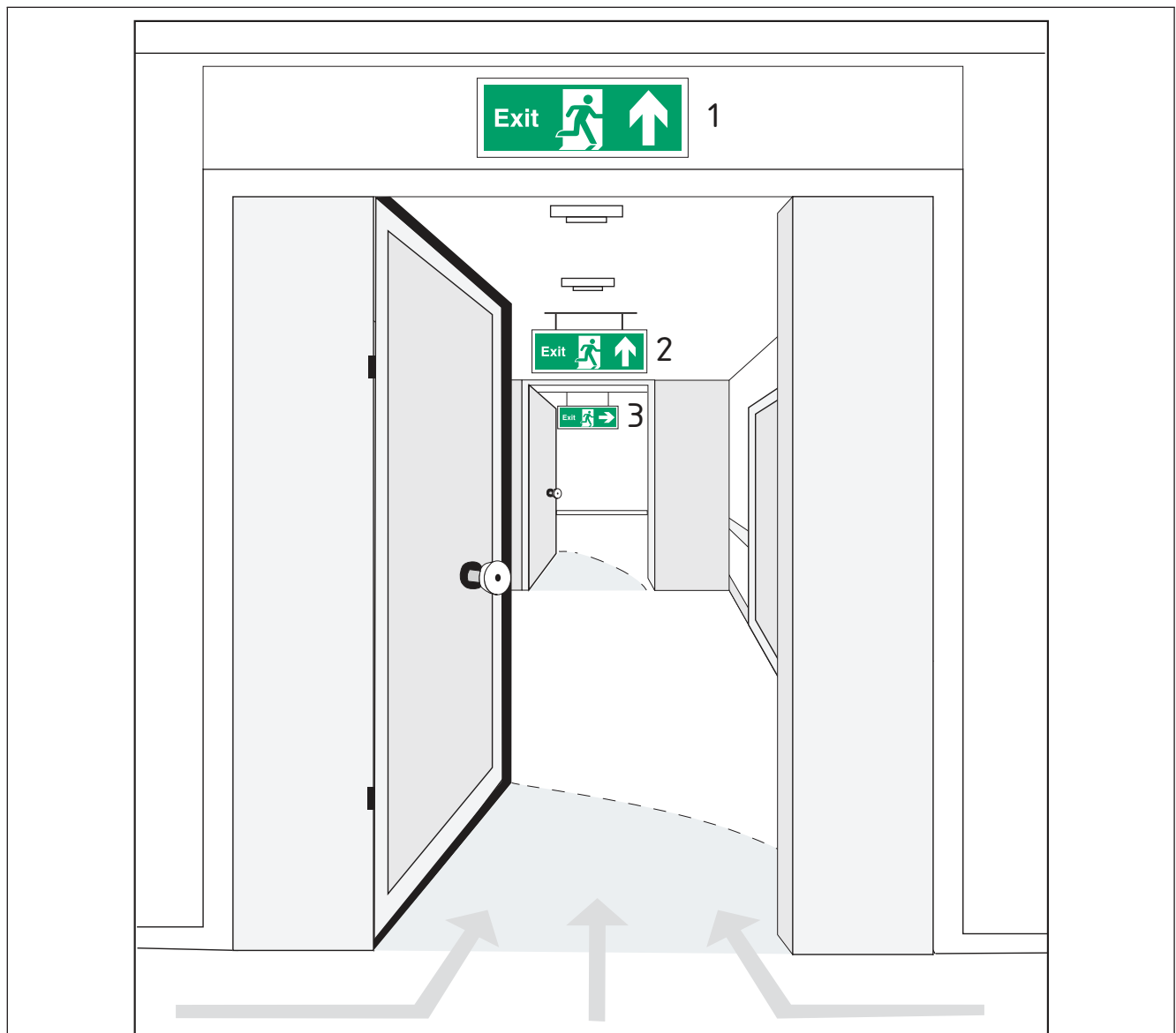
Figure A.13 Typical connecting corridor with right-turn juncture showing the correct use of escape route sign(s) with supplementary text
