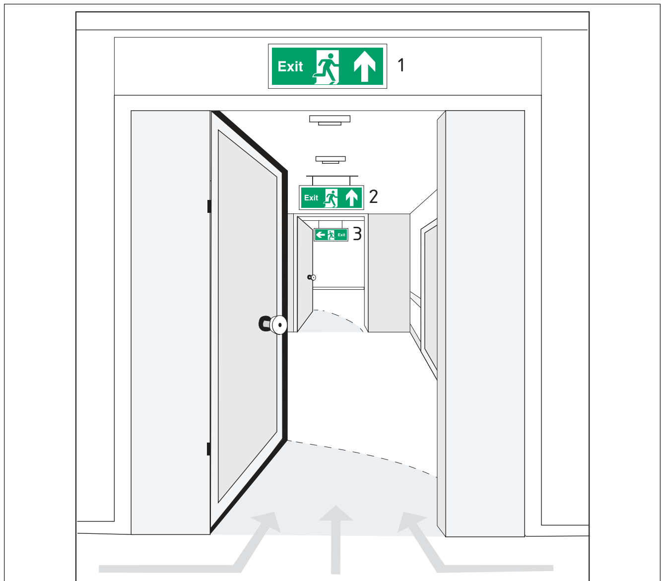
Figure A.12 Typical connecting corridor with left-turn juncture showing the correct use of escape route sign(s) and supplementary text
