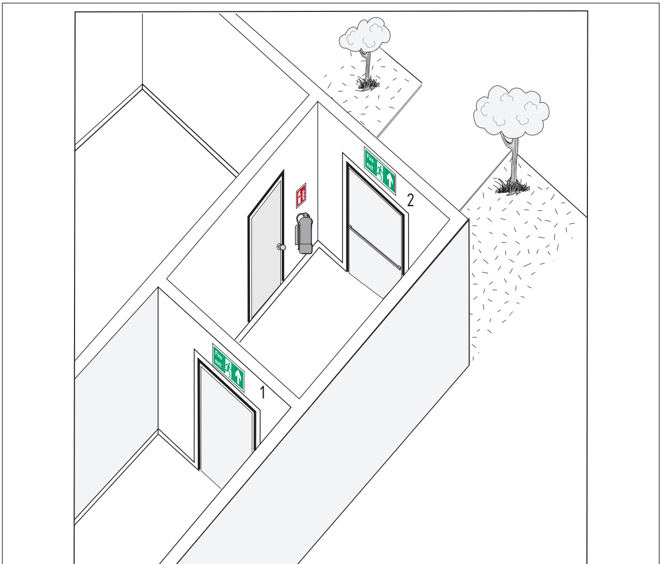
Figure A.2 Typical adjoining corridor to final fire exit showing the correct use of escape route sign(s) with supplementary text
