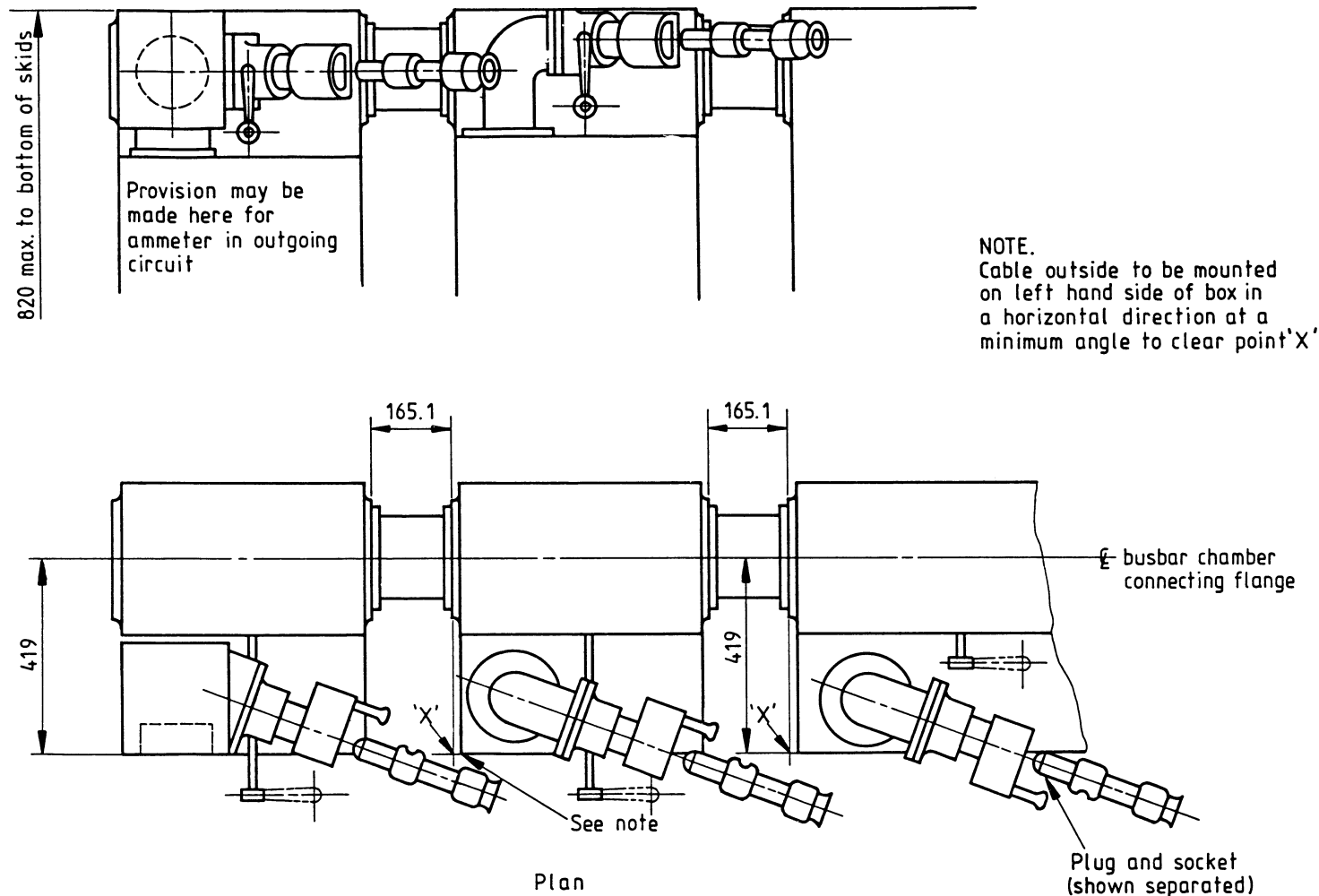
Figure 7 — Example of outgoing cable fittings
