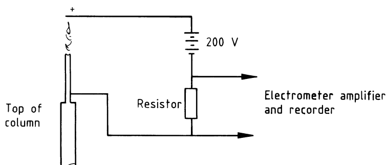
Figure D.1 — Flame ionization detector (schematic)
