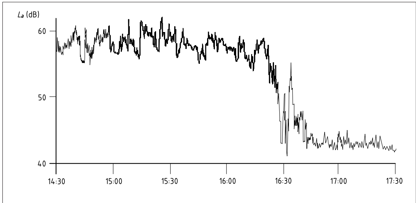
Figure A.8 Sound level variation with time
