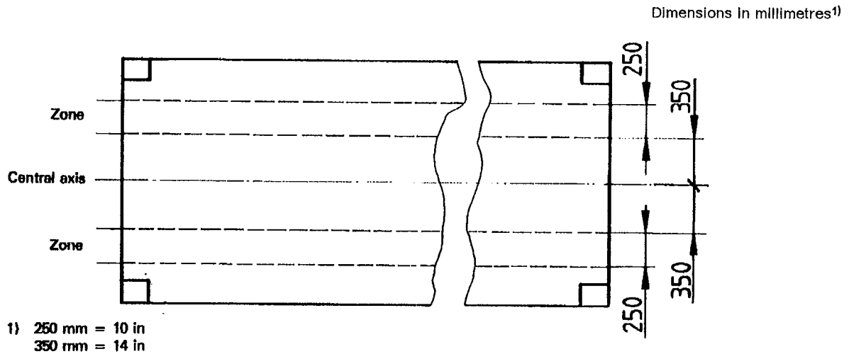
Figure B.1 — Zones for longitudinal members
