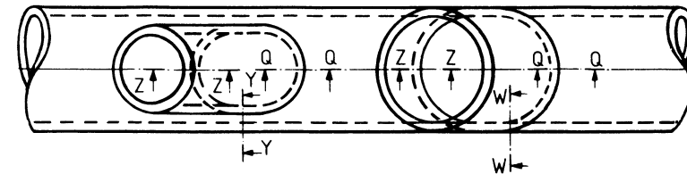
Figure 6 — Details of set-on branches
