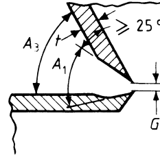
Section Z-Z at crotch of sloping branch
