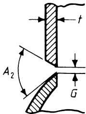
Section Y-Y at flank of unequal branch
