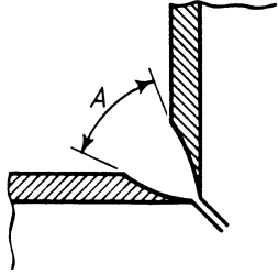
Section X-X at crotch of right angle branch
