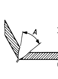
Section Q-Q at back of sloping branch
