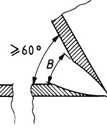
Section Z-Z at crotch of sloping branch
