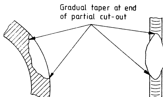
Figure 15 — Partial cut-out in rectification of faulty welds
