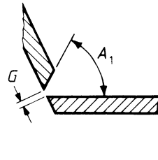
Section Q-Q at back of sloping branch
