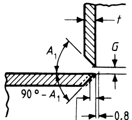
Section X-X at crotch of right angle branch
