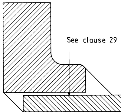
Figure 14 — "Slip-on" hubbed welded-on flange
