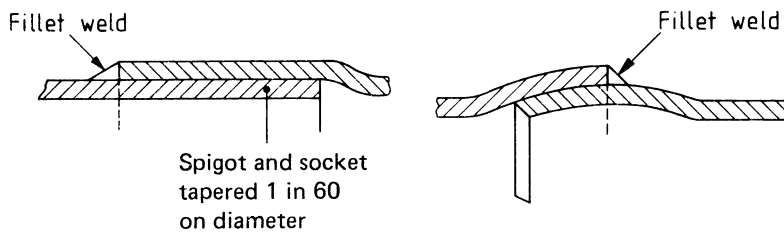
Figure 10 — Sleeve joints
