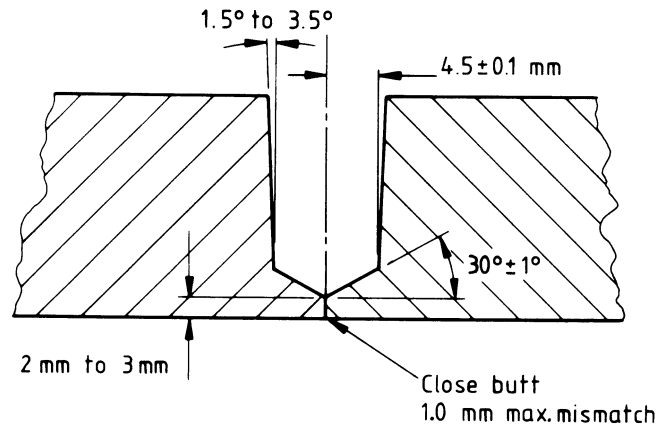
(a) For use with automatic TIG or MIG welding
