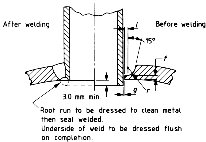
(b) Single-J preparation
