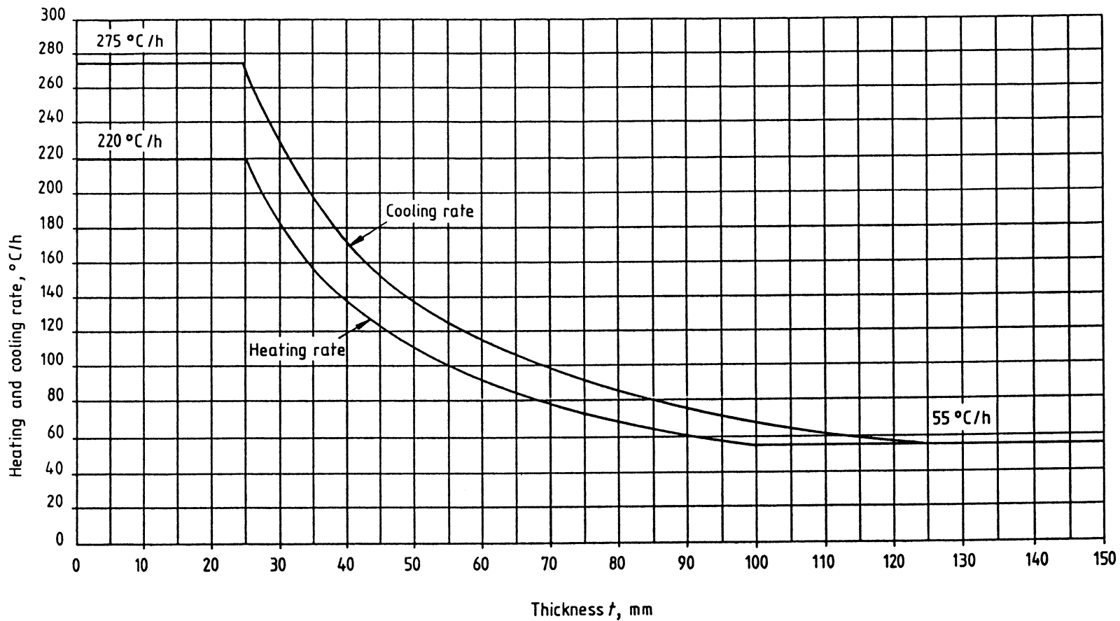
Figure 6 — Post-weld heat treatment heating and cooling rates for materials other than \frac{1}{2} Cr \frac{1}{2} Mo \frac{1}{4} V, 2\frac{1}{4} Cr 1 Mo, 1.25 Ni Cu Mo Nb and 9 Cr 1 Mo V Nb N steels
