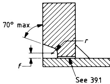
Figure 27 — Typical “face and fillet” welded-on flange
