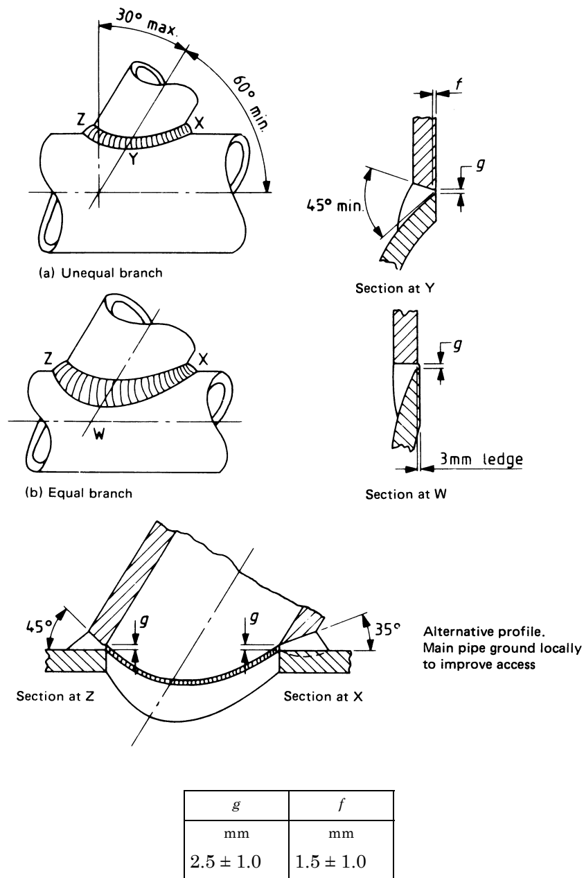
Figure 18 — Typical preparation and assembly of set-on sloping branches without backing
