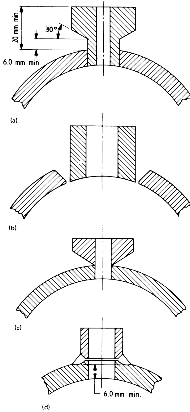
Figure 23 — Typical small bore connections
