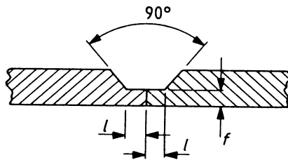
(c) Single-V with lands
