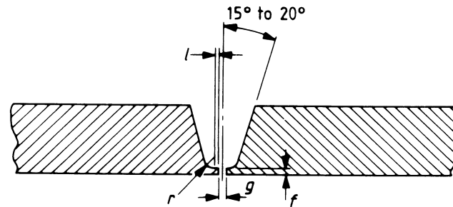
(a) Single-J with lands, any thickness
