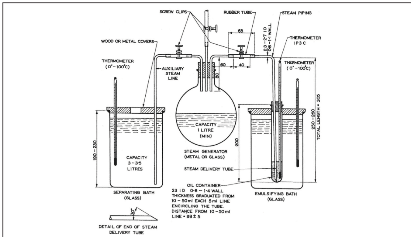
Figure 1 Apparatus for steam emulsion test, self-generating steam supply
