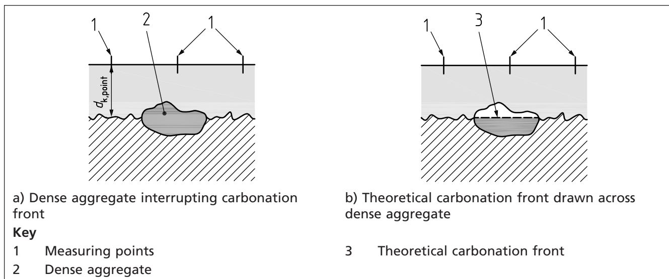
Figure 2 Procedure for obtaining the carbonation depth where the point falls within a dense aggregate particle
