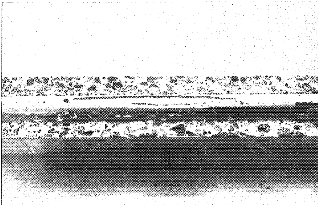
(b) Sectioned beams with grouting fault exposed
