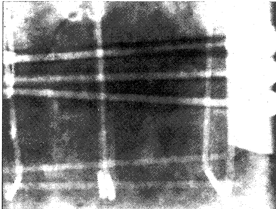
(a) Radiograph of the anchorage of a prestressed concrete beam shown in (b)
