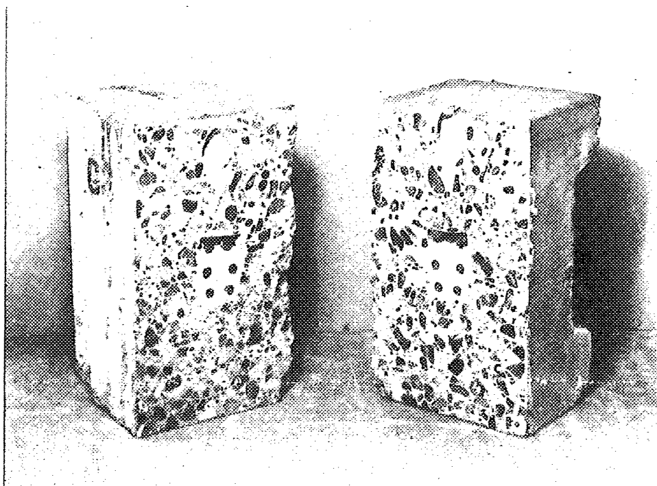
(b) Sawn section of prestressed beam end
