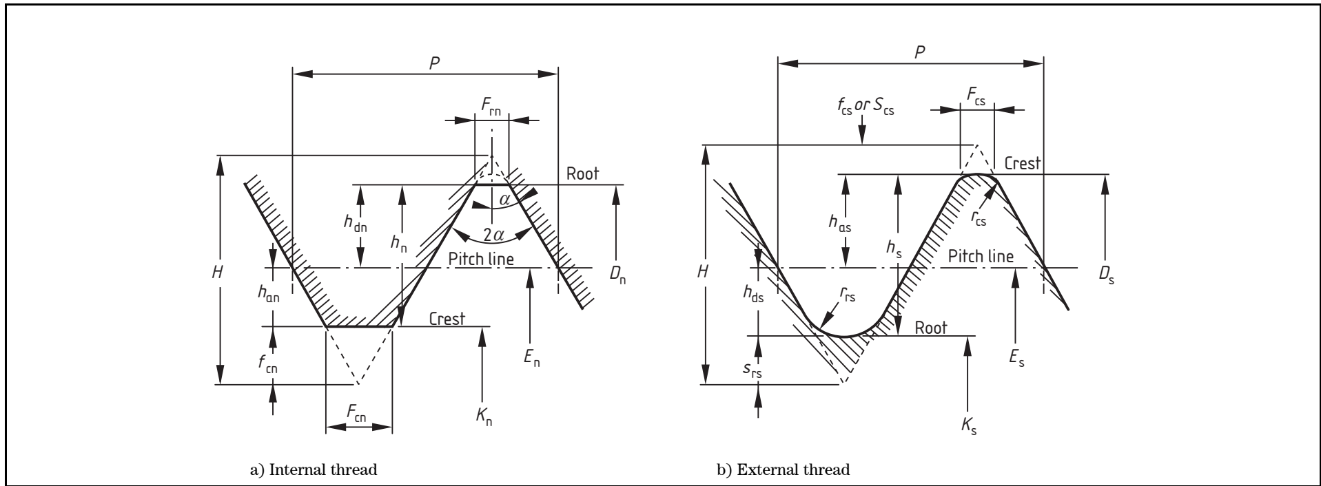
Figure D.1 General symbols
