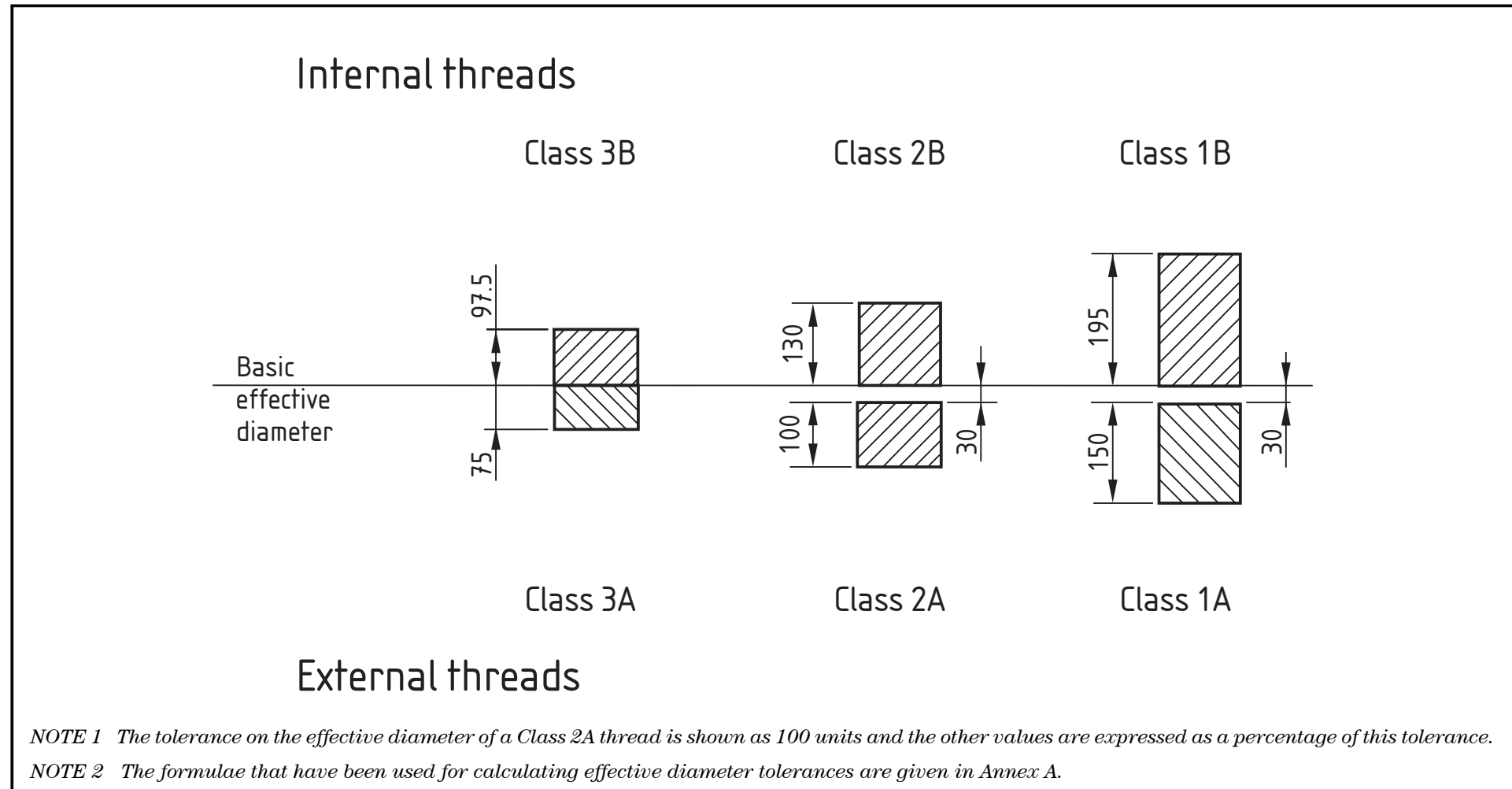
Figure 4 Classes of unified screw threads – Effective diameter tolerance zones of finished uncoated threads
