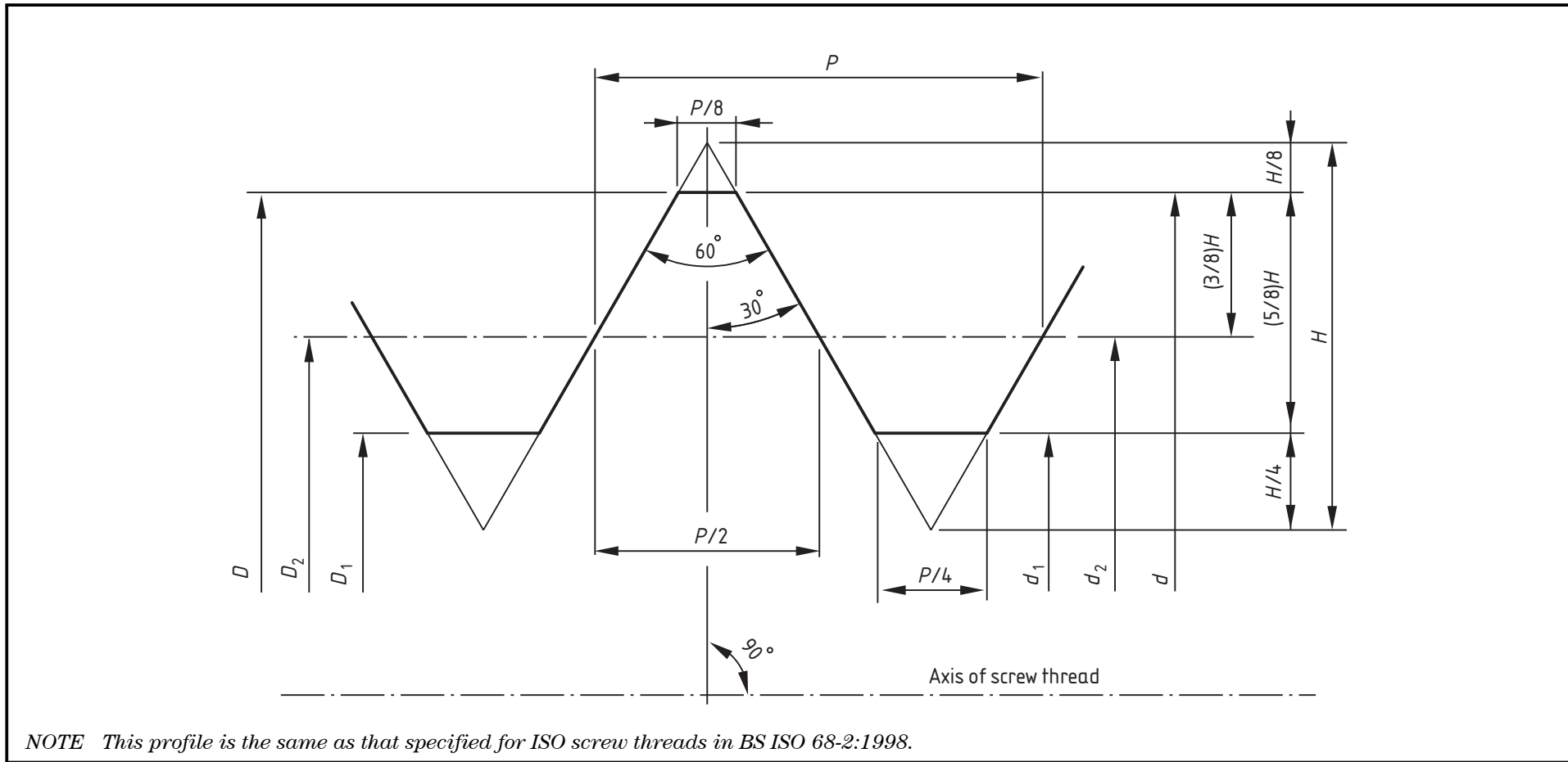
Figure 1 Basic profile of unified screw threads
