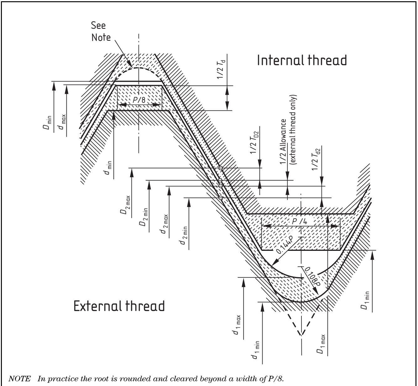
Figure 7 Tolerance zones for unified threads, Class 2A external thread and Class 2B internal thread
