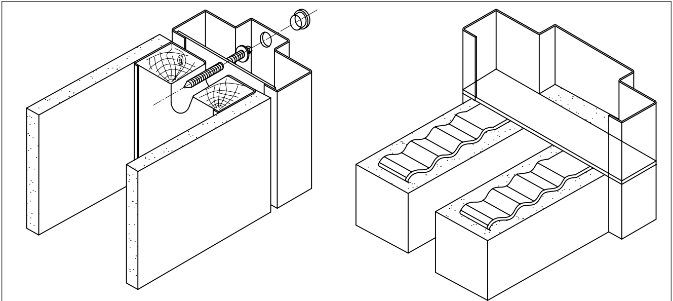
Figure 10 Typical frame fixing methods (2 of 2)
