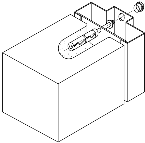
Figure 10 Typical frame fixing methods (1 of 2)
