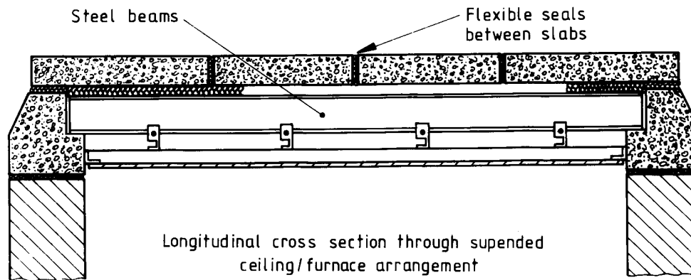
(c) Longitudinal cross section through suspended ceiling/furnace arrangement
