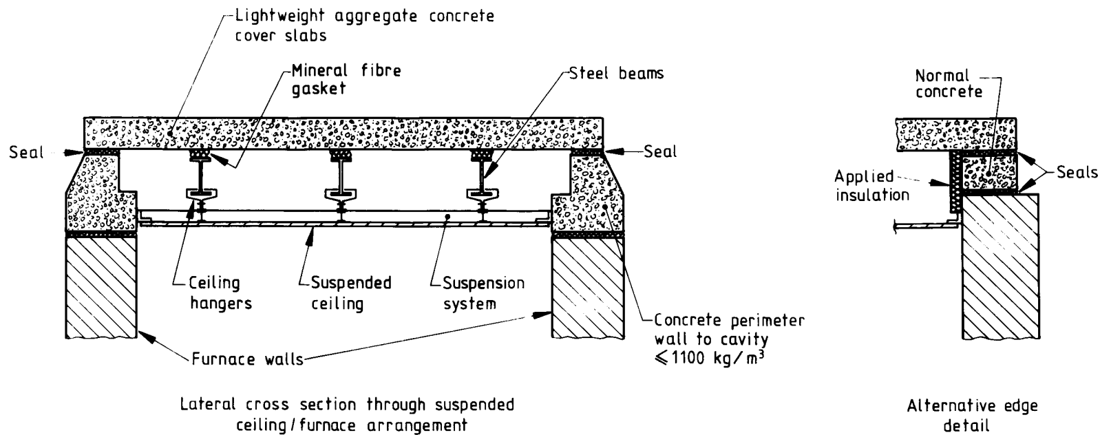
(a) Lateral cross section through suspended ceiling/furnace arrangement
