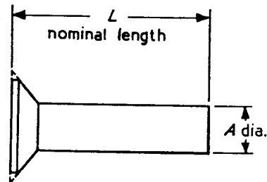
Figure 4 — Rivet dimensions
