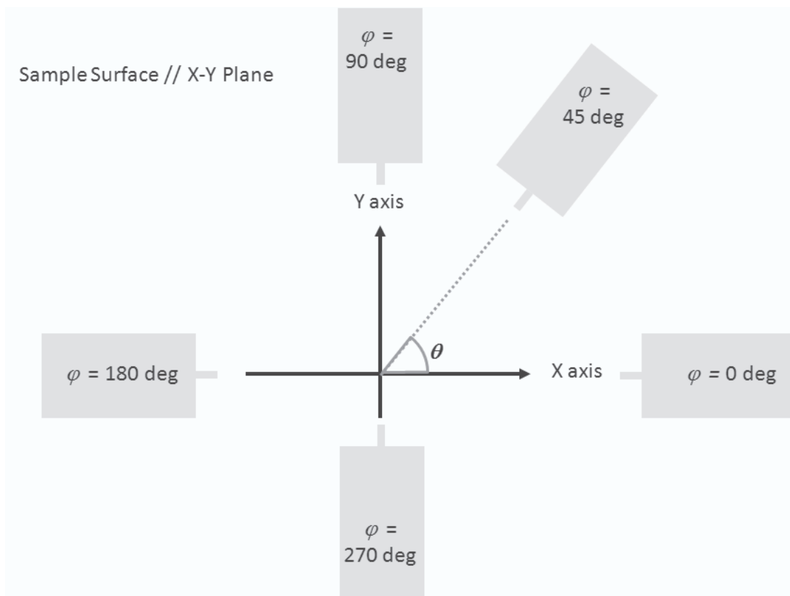
Figure A.2 — Geometrical arrangement of the SPM probe in the X-Y plane, indicating the angle between the probe tip and the X axis
