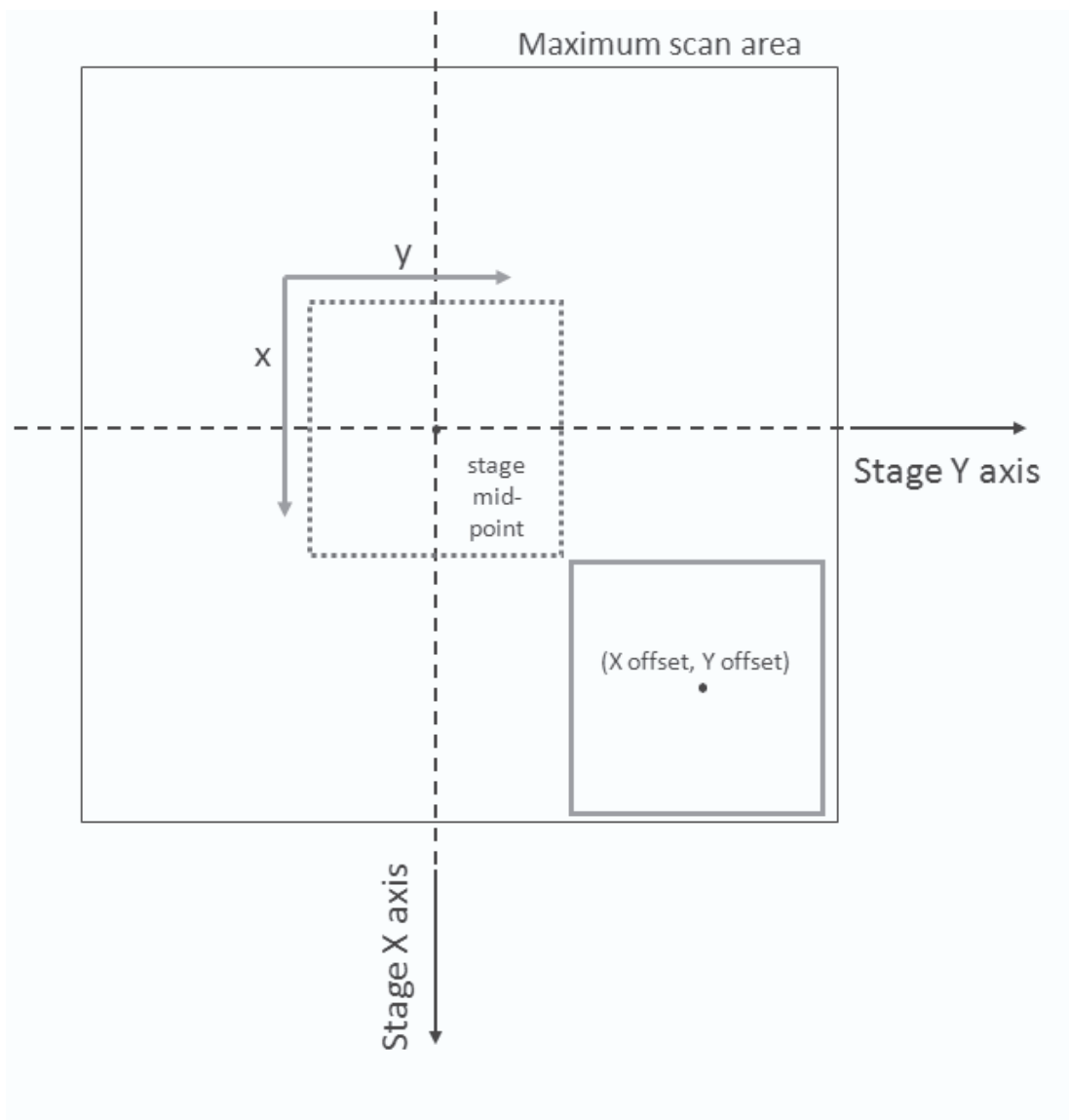
Figure B.1 — Schematic illustration of the data acquisition area scanned by an SPM probe using the sample stage X-Y coordinates or global coordinates
