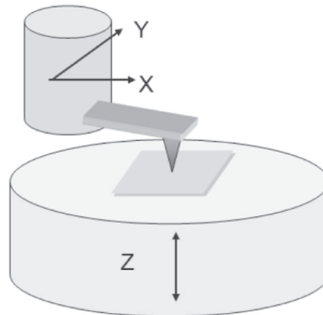
d) Sample scanned in Z direction and probe scanned in X and Y directions
