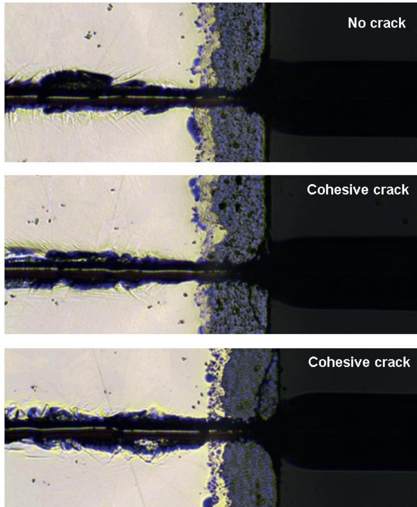
Figure C.1 — Optical micrographs on the cross-section of plasma sprayed TiO 2 coatings scratched at a constant load of 3 N, which tested in Finland
