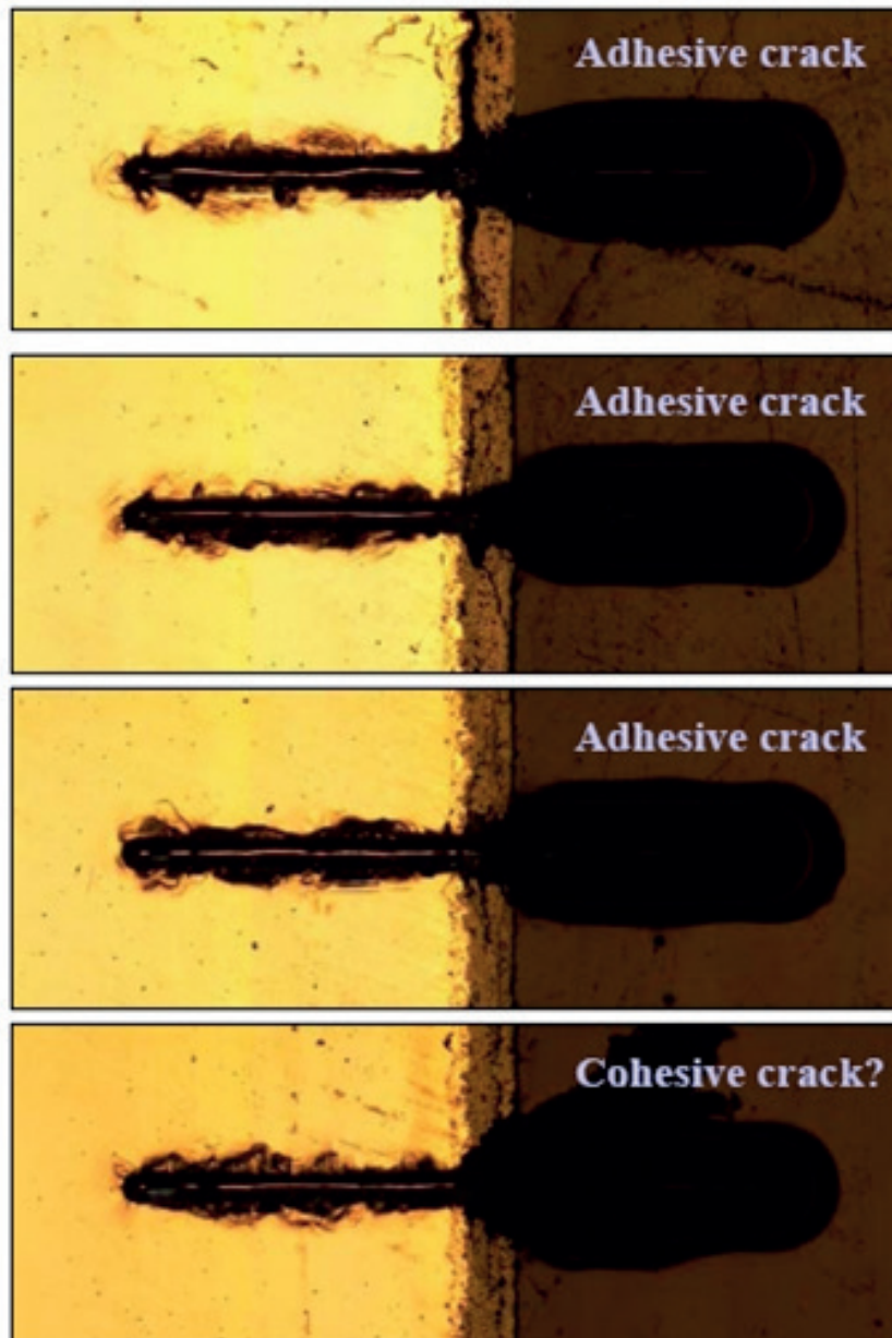
Figure C.7 — Optical micrographs on the cross-section of plasma sprayed TiO 2 coatings scratched at a constant load of 10 N, which tested in Japan
