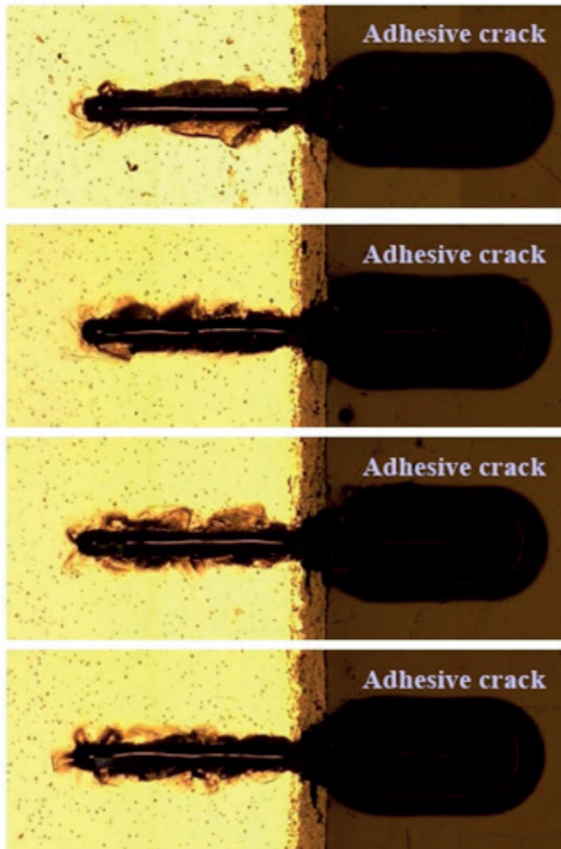
Figure C.9 — Optical micrographs on the cross-section of plasma sprayed TiO 2 coatings scratched at a constant load of 15 N, which tested in Japan
