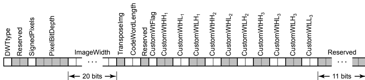
Figure 4-7: Segment Header Part 4
