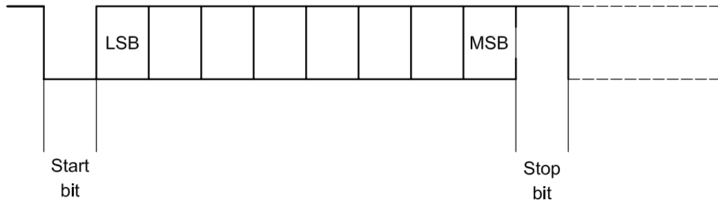
Figure 6 — Byte format of bidirectional communication ACL
