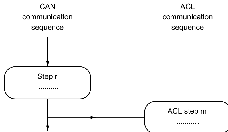
Figure 3 — Integration of ACL communication into deployment process
