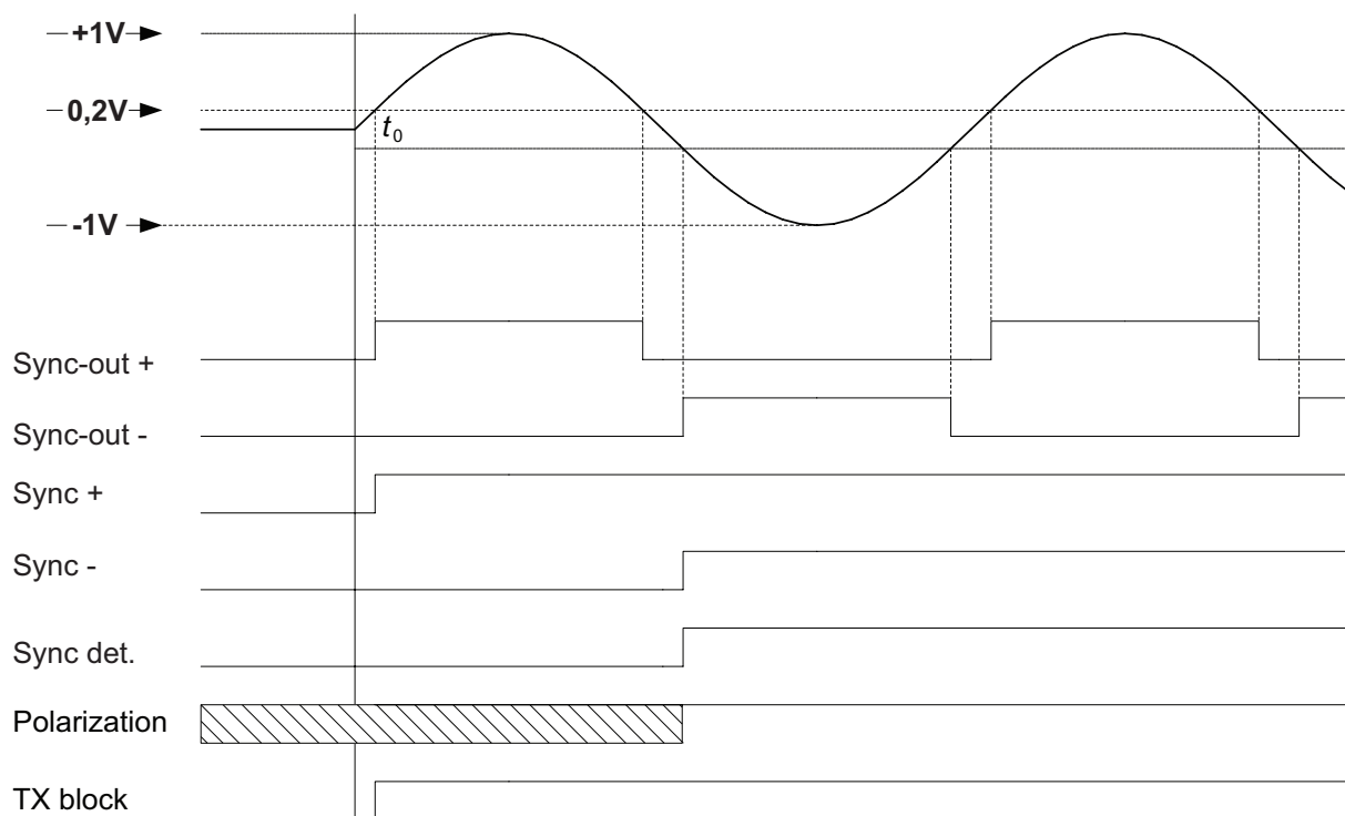
Figure 8 — Synchronization pulse rising edge
