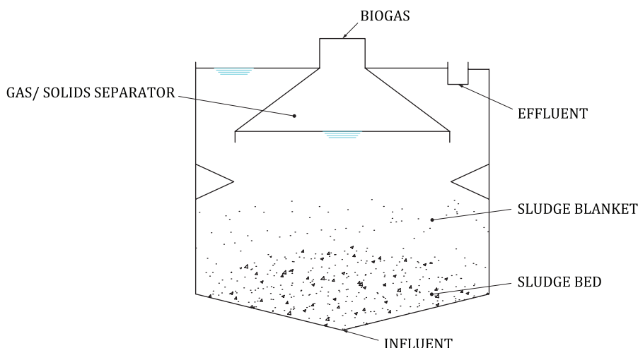
Figure B.15 — Upflow anaerobic sludge blanket reactor
