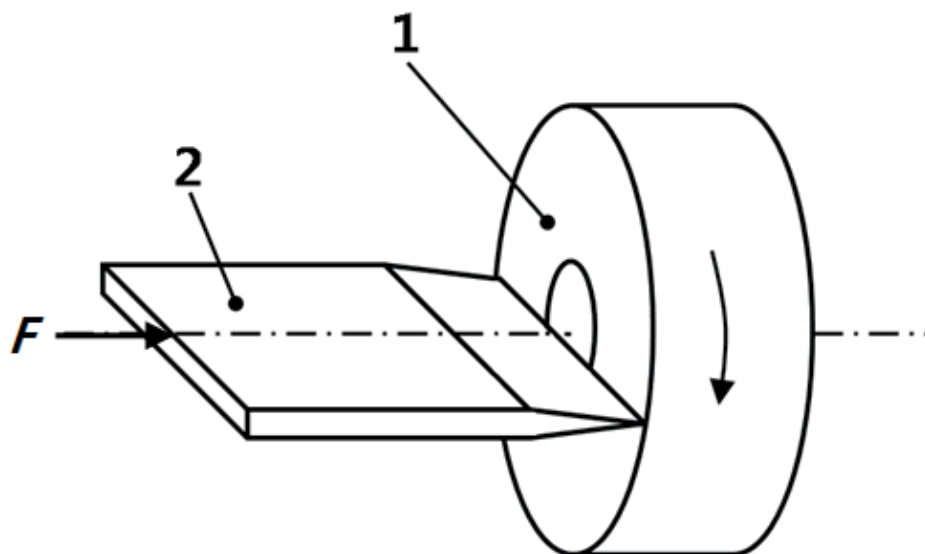
Figure 8 — Test pieces and abrasants inside a rotating drum
