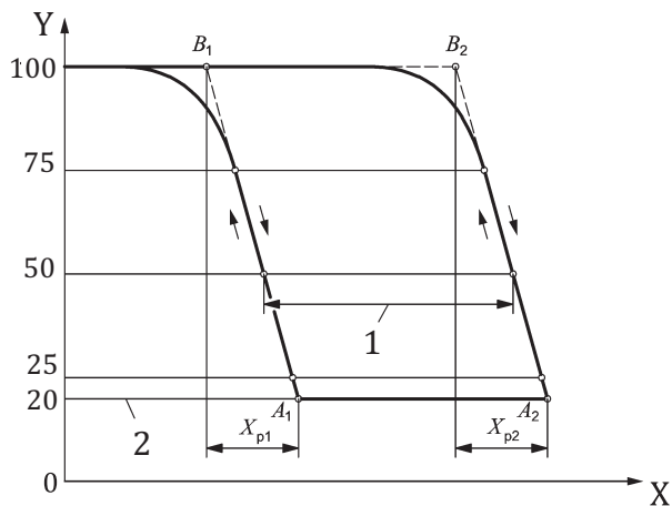
a) Modulating thermostat
