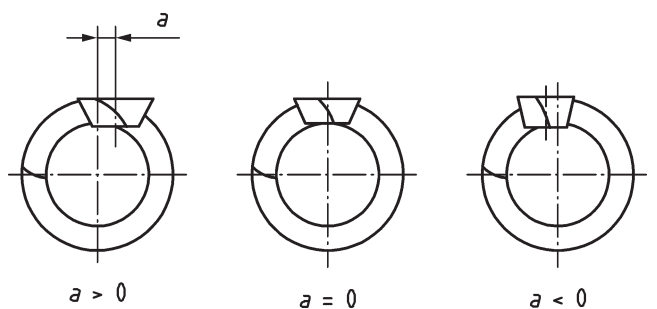
a) Left-hand pinion mated with right-hand wheel
