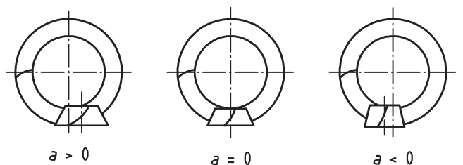
b) Right-hand pinion mated with left-hand wheel
