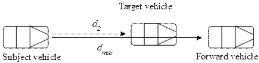
Figure 13 — Straight road lateral offset discrimination ability test
