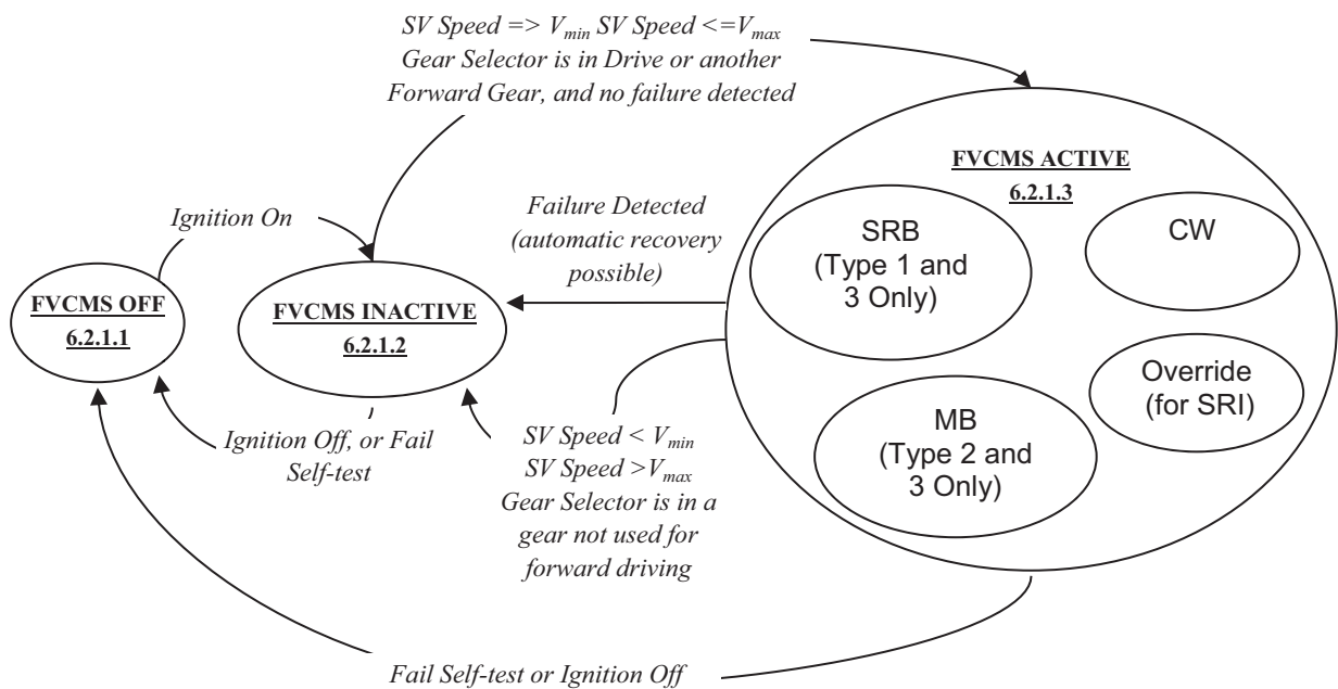
Figure 2 — FVCMS State Transition Diagram
