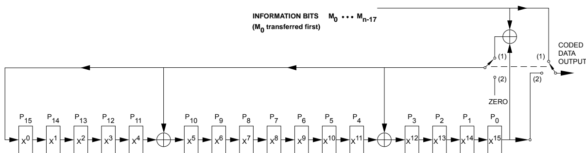
Figure 4-5: Logic Diagram of the Encoder
