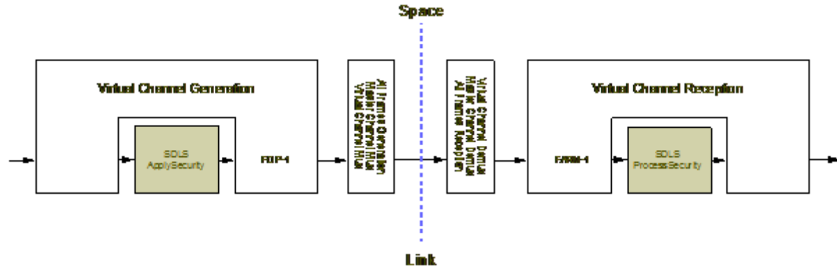
Figure 6-3: Order of Processing between TC, COP-1, and SDLS Functions
