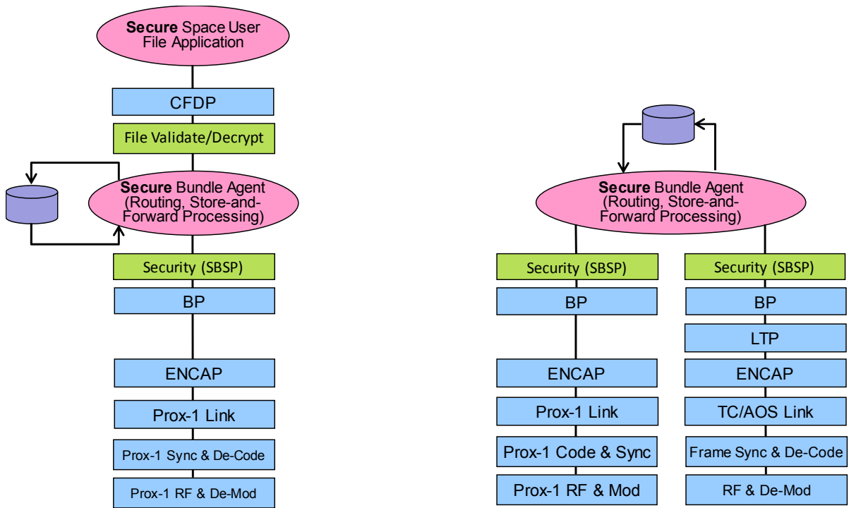
a) SSI Secure Space User Node Proximity Link with Bundle Routing
