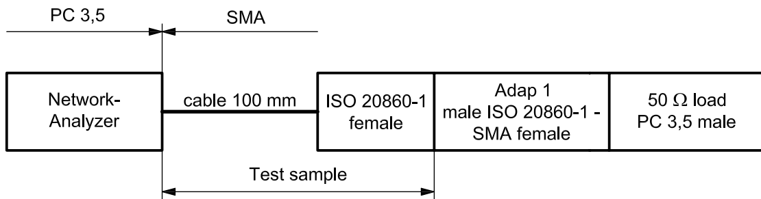
Figure 1 — Test configuration for female connector
