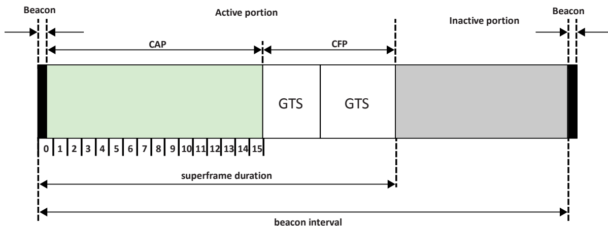
Figure 2-1: IEEE 802.15.4 Superframe
