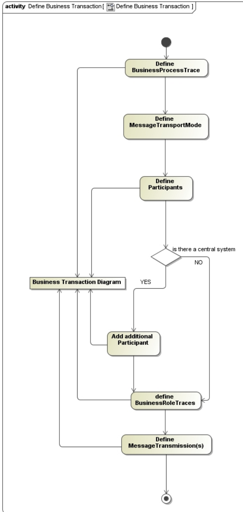
Figure 3 — Define BusinessTransaction
