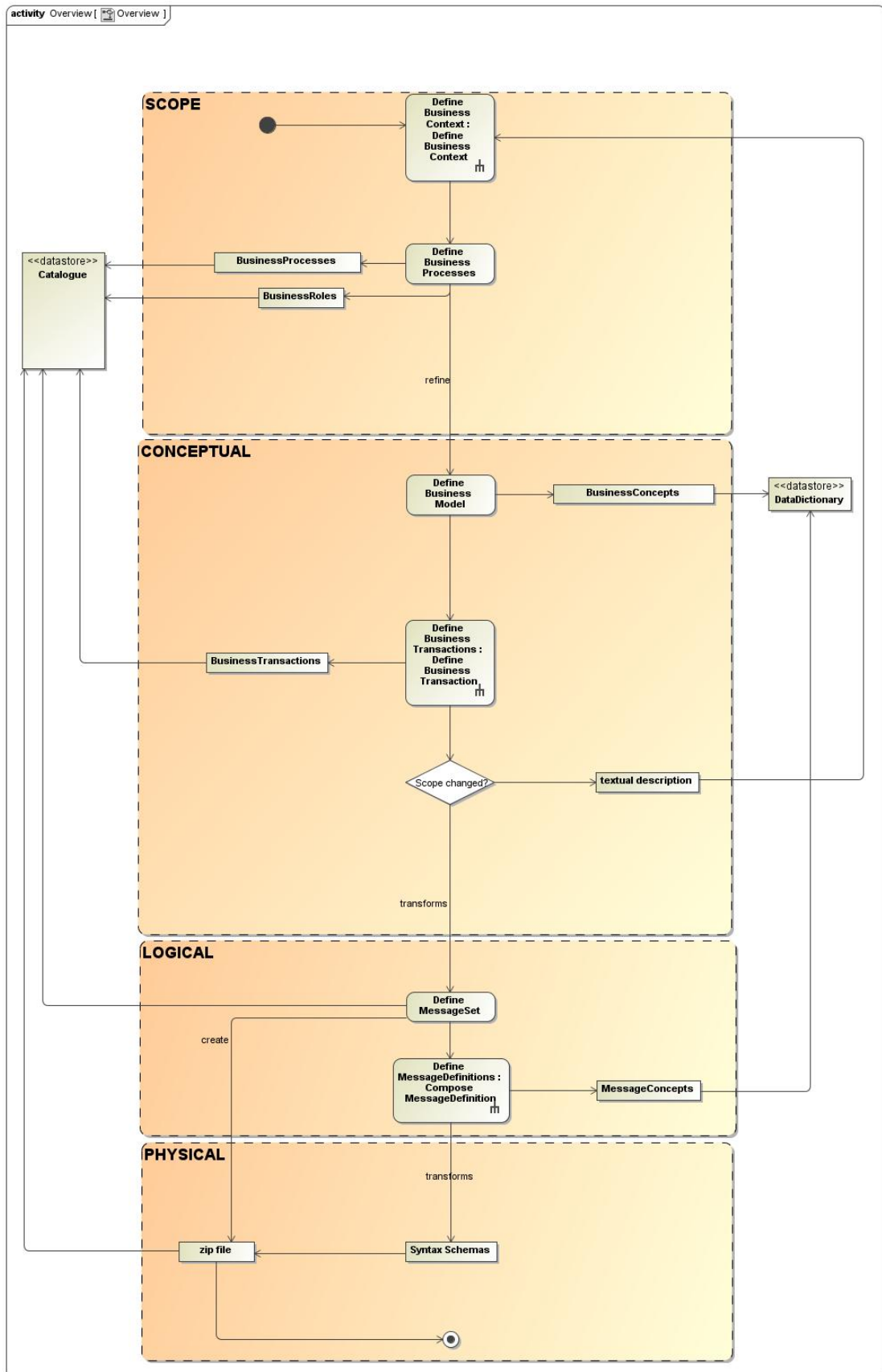
Figure 1 — High level workflow activity diagram
