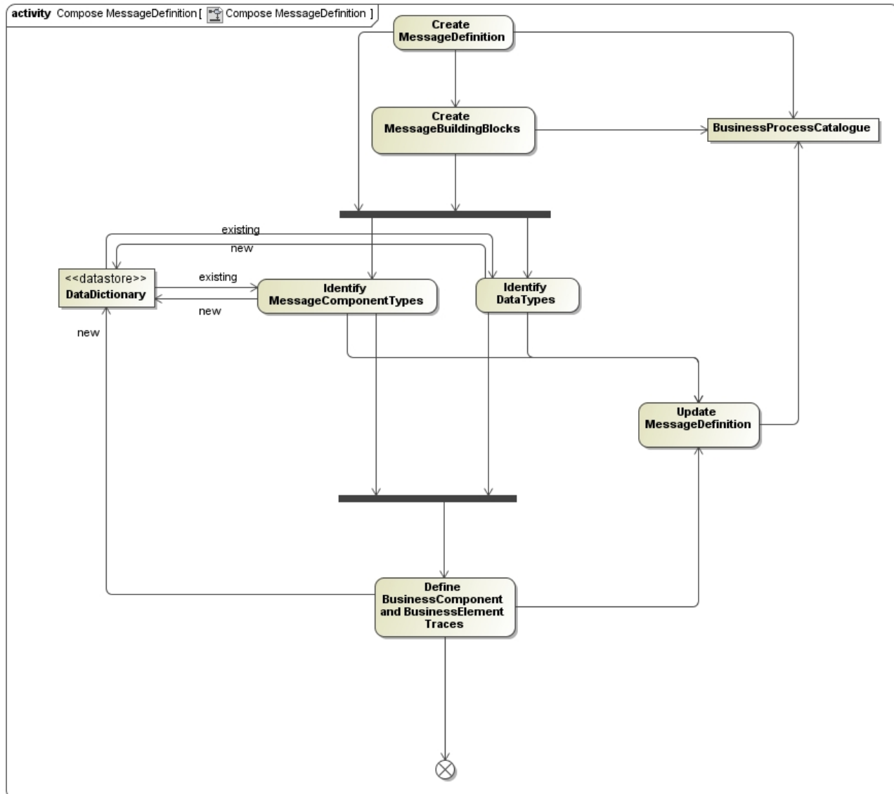
Figure 4 — Compose MessageDefinition
