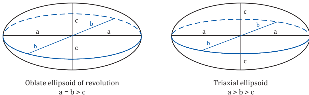
Figure D.1 — Oblate and triaxial ellipsoids
