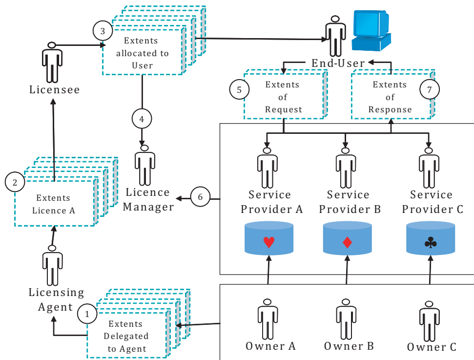
Figure C.5 — Workflow licensed access to content from multiple providers
