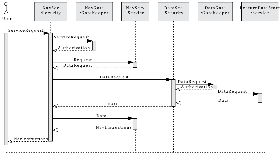
Figure 4 — Sequence diagram for a two-stage geoServer interaction
