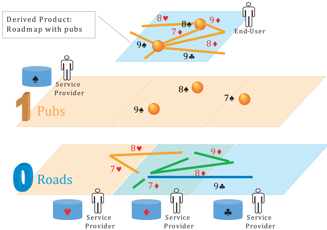
Figure C.7 — Derived resource adding content
