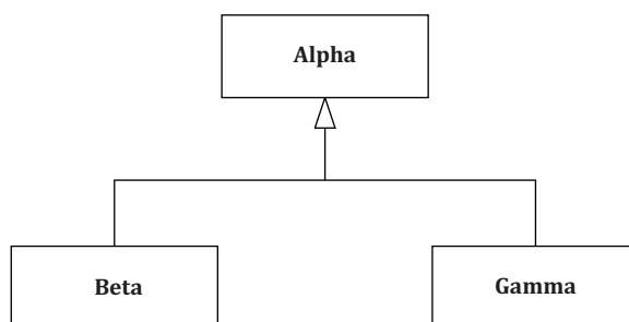
Figure C.4 — UML generalization
