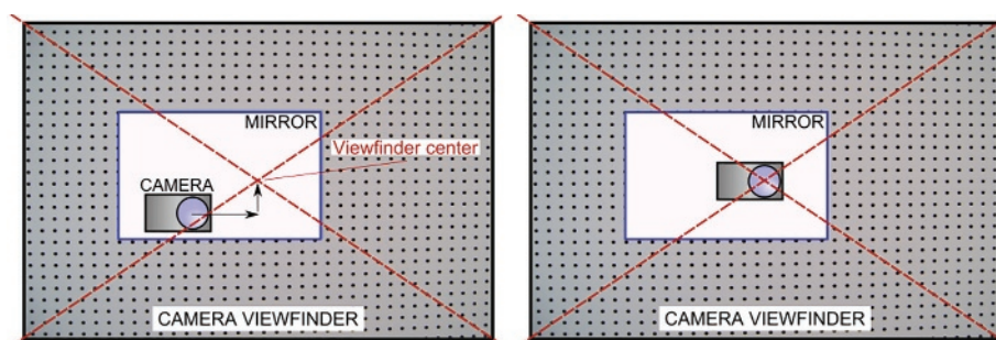
Figure 6 — Alignment of the camera with the target plane using a mirror
