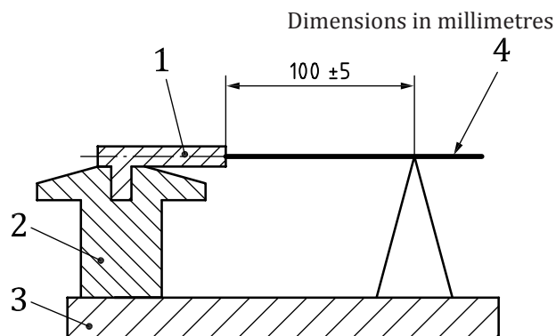
Figure 4 — Straight connector mounting for combined temperature/humidity/vibration test
