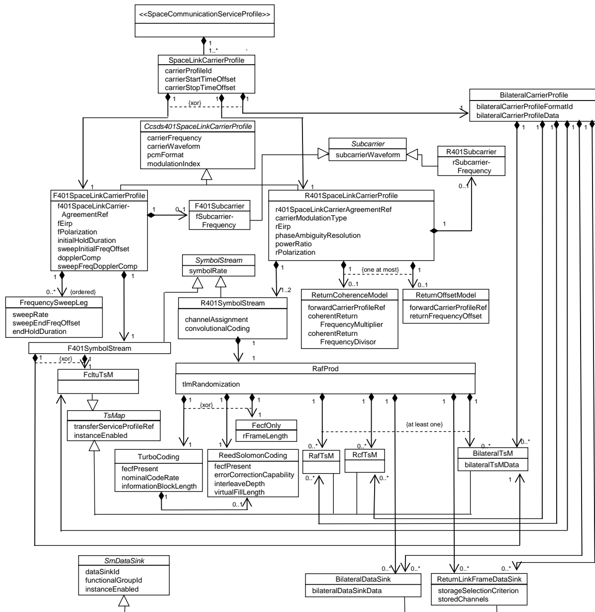
Figure 5-2: <<SpaceCommunicationServiceProfile>> Stereotype Structure Class Diagram
