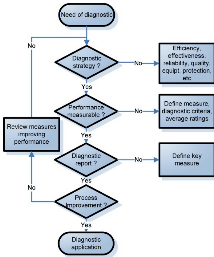
Figure B.1 — Diagnostic strategy
