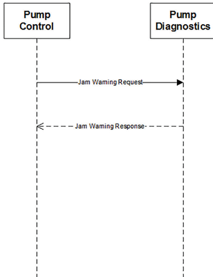
Figure C.1 — Jam detection information exchange
