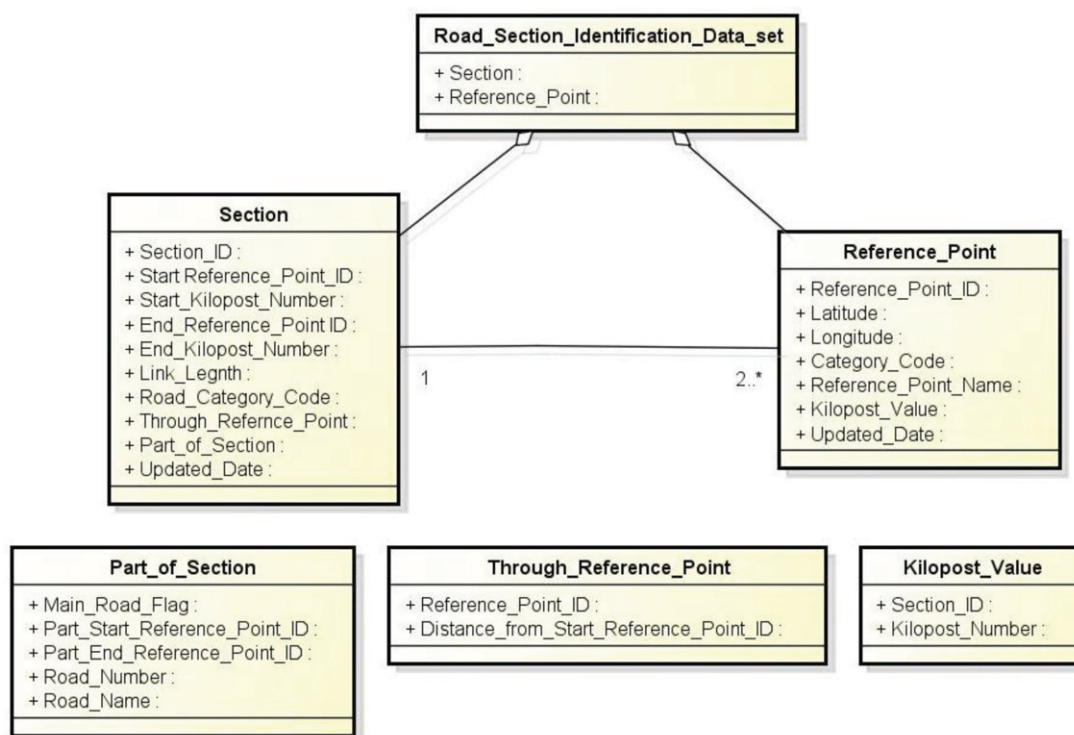
Figure H.1 — Structure of road section referencing
