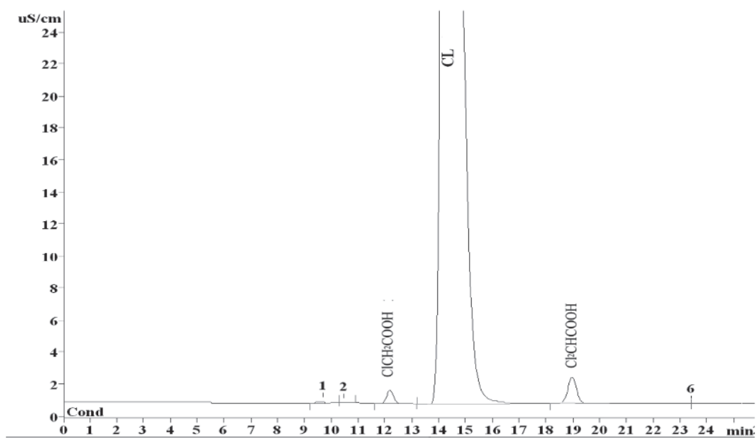
Figure A.1 — A typical IC chromatogram for monochloroacetic acid and dichloroacetic acid (on IC condition 1)
