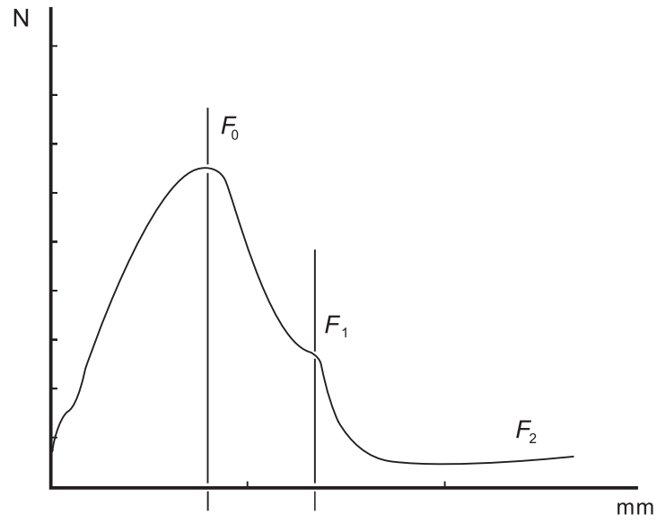
Figure B.3 — Diagram of the typical puncture force of the needle ( F_0 , F_1 , F_2 )
