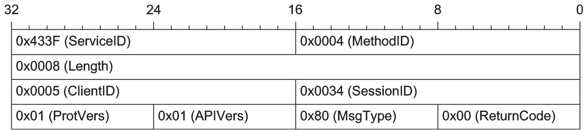
Figure 10 — SetCamControlAccess response
