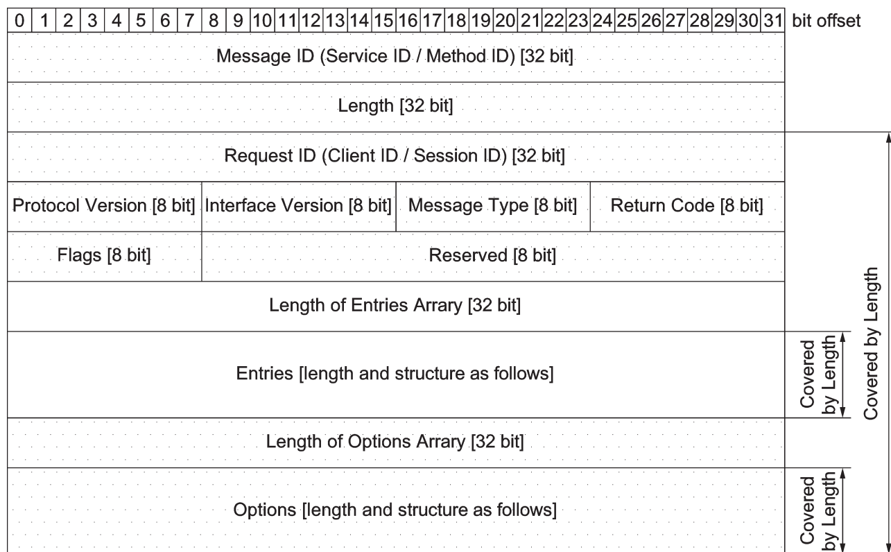
Figure 9 — SOME/IP service discovery packet format
