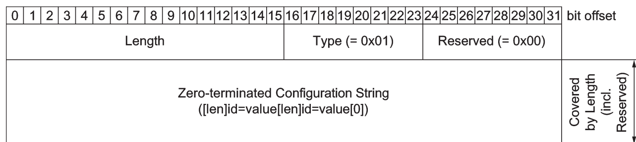
Figure 12 — SOME/IP SD configuration option layout
