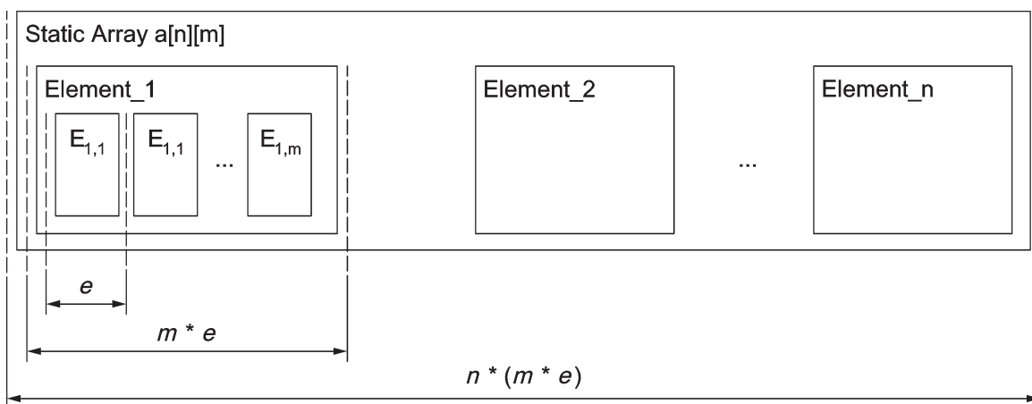
Figure 6 — Fixed-size multidimensional array memory layout
