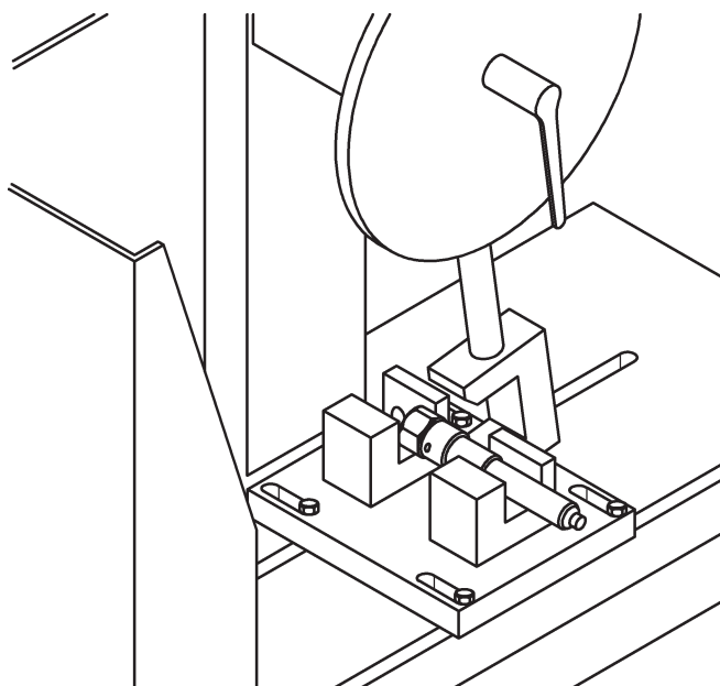
Figure A.5 — Impact point on flexible hose assembly
