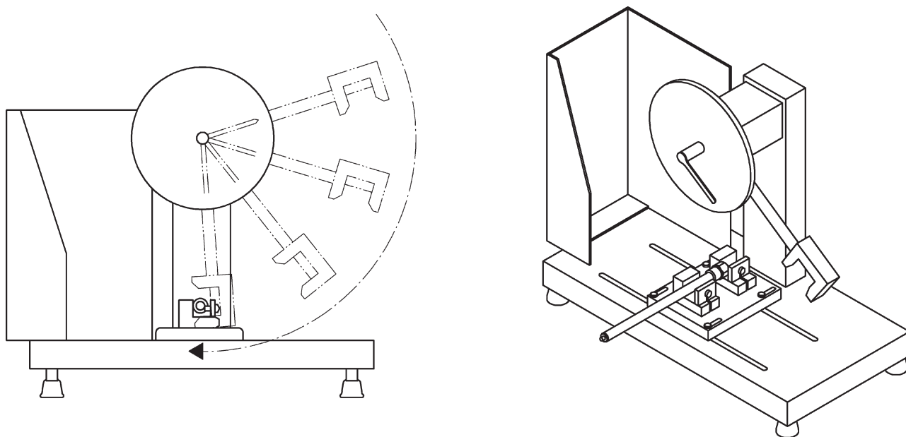
Figure A.4 — Test apparatus and set up
