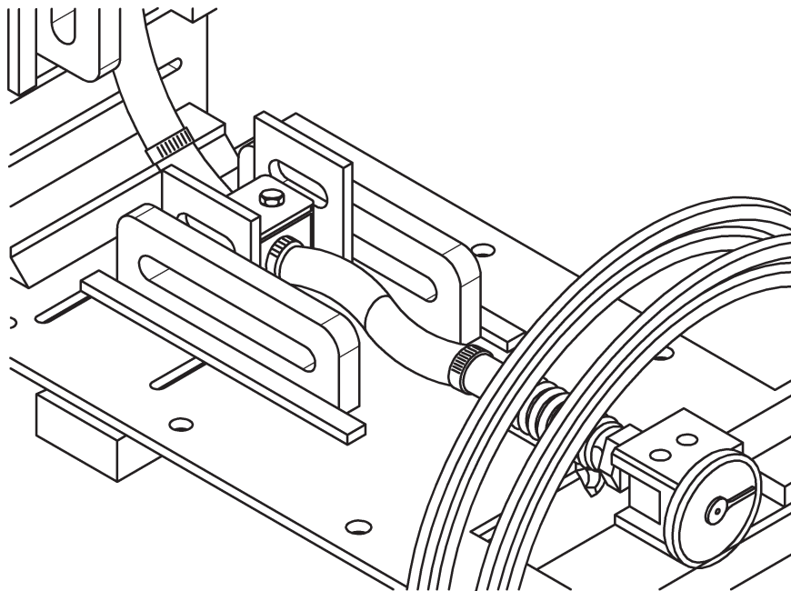
Figure A.7 — Sinusoidal movement of \pm 90^\circ about the rotating x-axis
