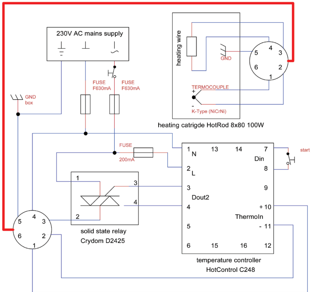
Figure A.1 — Connection diagram
