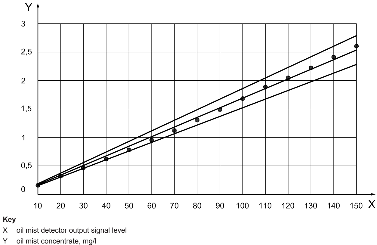
Figure A.2 — Sample of calibration result of oil mist detector output signal
