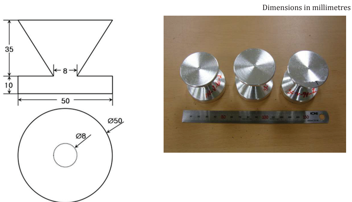
Figure 1 — Shape and dimension of the test specimen obtained by machining from ingots
